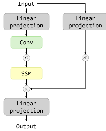
FIG. 4. Mamba block.
