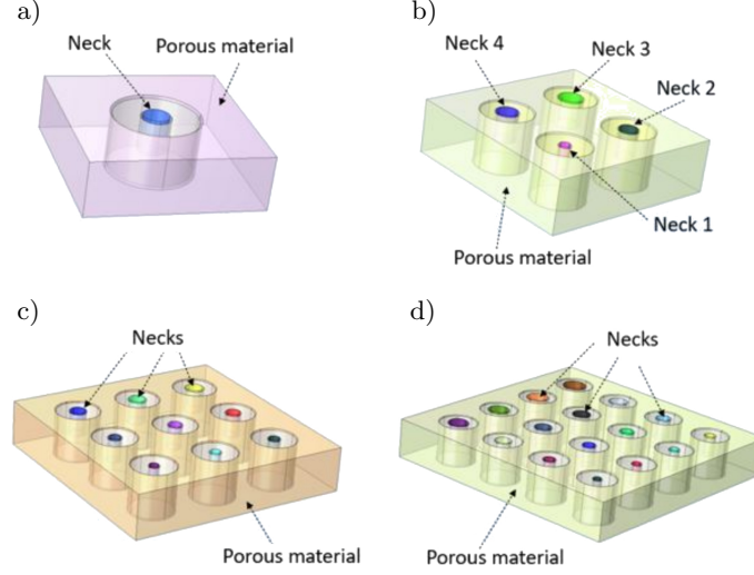
FIG. 1. Acoustic metamaterial based on porous layer with embedded multiple resonators: a) one periodic resonator, b) four periodic resonators, c) nine periodic resonators, d) sixteen periodic resonators.
