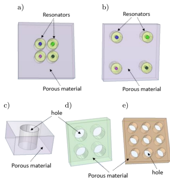
FIG. 10. Geometrical models of: a) porous layer with four resonators, L = 45\text{ mm} , b) porous layer with four resonators, L = 110\text{ mm} , c) porous layer with one perforation, d) porous layer with four perforations, e) porous layer with nine perforations.
