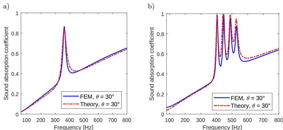
FIG. 9. Sound absorption coefficient for oblique incidence: a) one embedded resonator, b) four embedded resonators.
