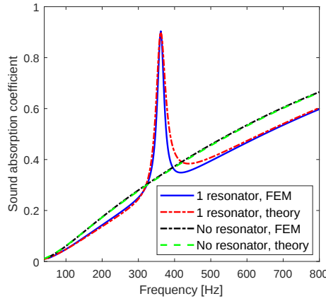
FIG. 5. Comparison of the sound absorption coefficient of the metamaterial with one embedded resonator.
