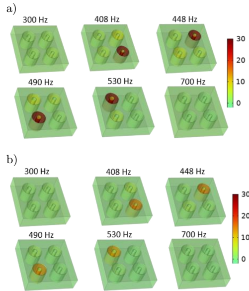
FIG. 17. Total RMS acoustic pressure [Pa]: a) \theta = 0^\circ , b) \theta = 75^\circ .
