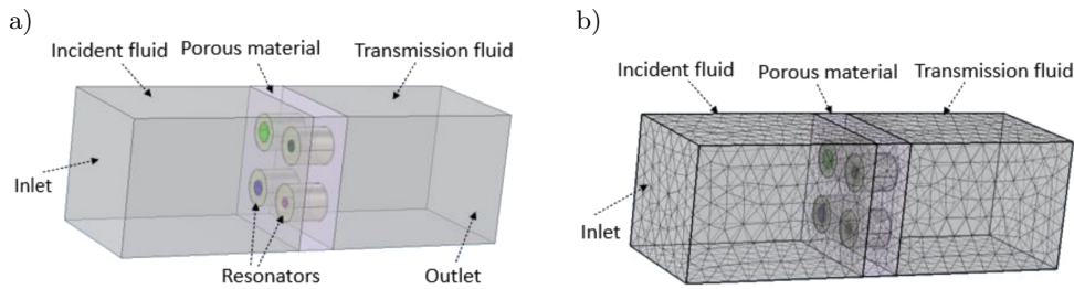
FIG. 2. PUC of the metamaterial: a) geometry with four HR, b) mesh with four HR.
