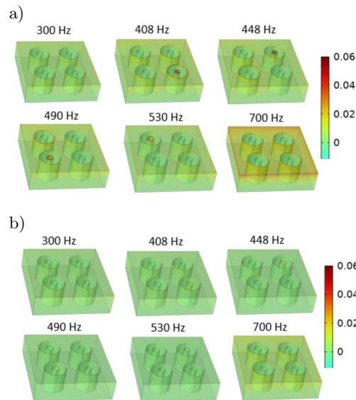
FIG. 19. Acoustic power dissipation density [ \text{W}/\text{m}^3 ]: a) \theta = 0^\circ , b) \theta = 75^\circ .
