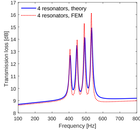
FIG. 8. Comparison of the transmission loss of the metamaterial with four embedded resonators.
