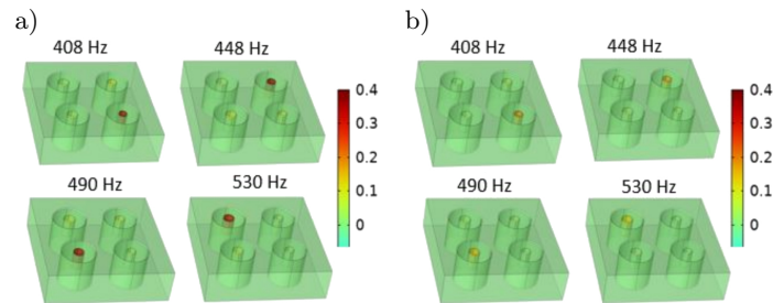
FIG. 18. Total acoustic velocity [m/s]: a) \theta = 0^\circ , b) \theta = 75^\circ .
