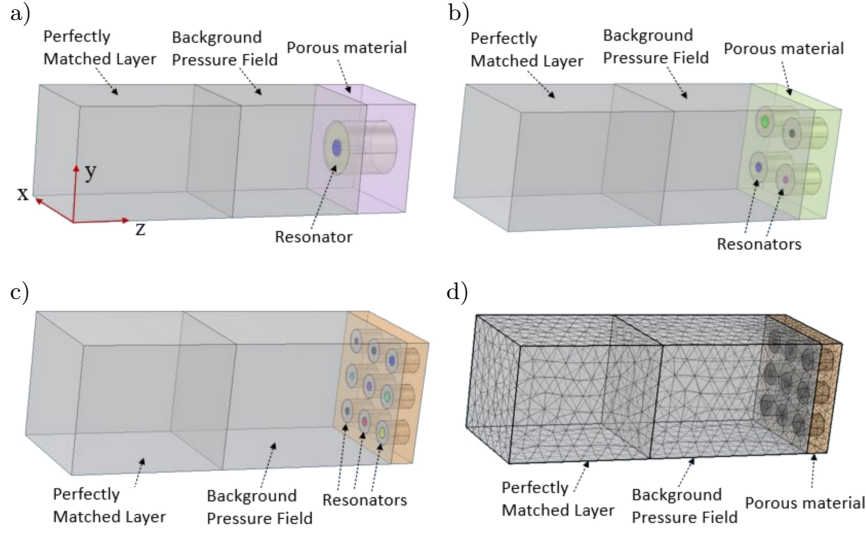
FIG. 3. PUC of the metamaterial for sound absorption estimation: a) PUC with 1 HR, b) PUC with 4 HR, c) PUC with 9 HR, d) mesh with 9 HR.
