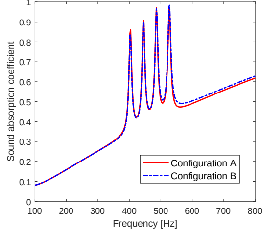
FIG. 11. Sound absorption coefficient.
