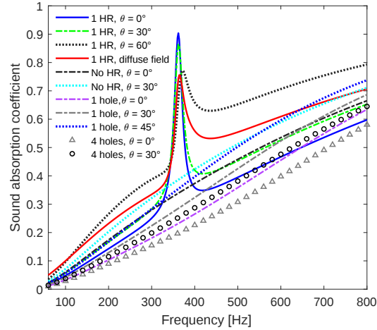
FIG. 12. Sound absorption coefficient of the metamaterial.
