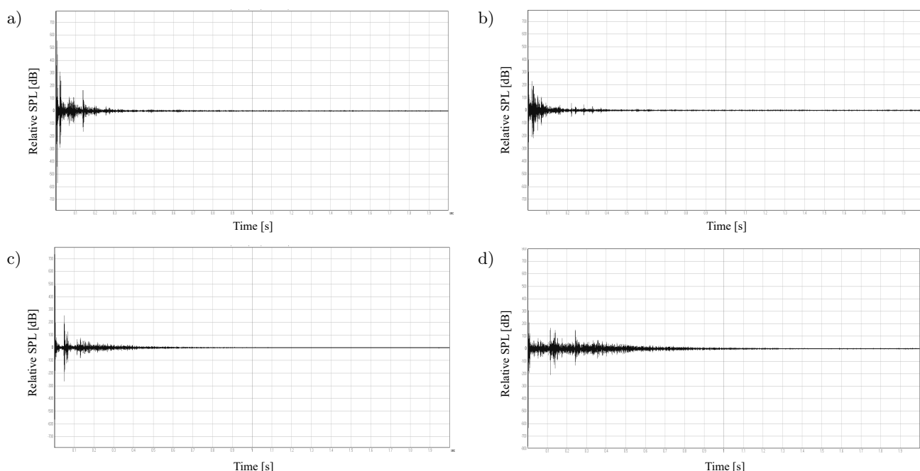
FIG. 4. Impulse responses at 1000 Hz for each of the four outdoor sites measured at a source-to-receiver distance of about 20 m: a) L-shaped, b) linear-shaped, c) U-shaped, d) square-shaped.
