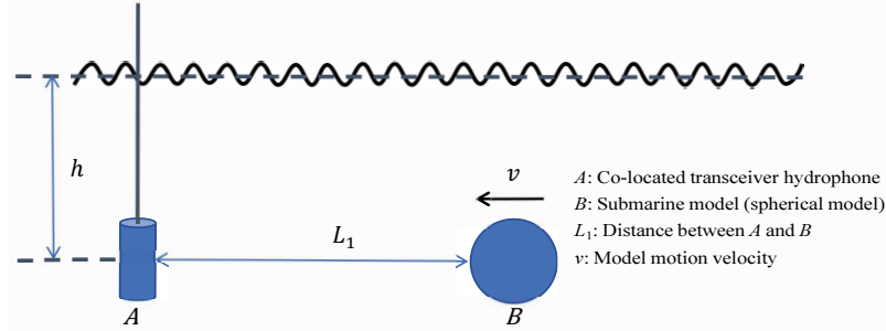
FIG. 3. Experimental deployment.
