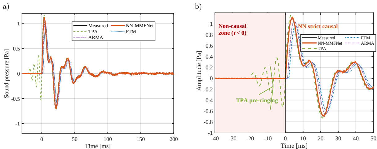
FIG. 10. Transient impulse response and causal verification: a) global transient impulse response, b) causality check (zoom at impact).
