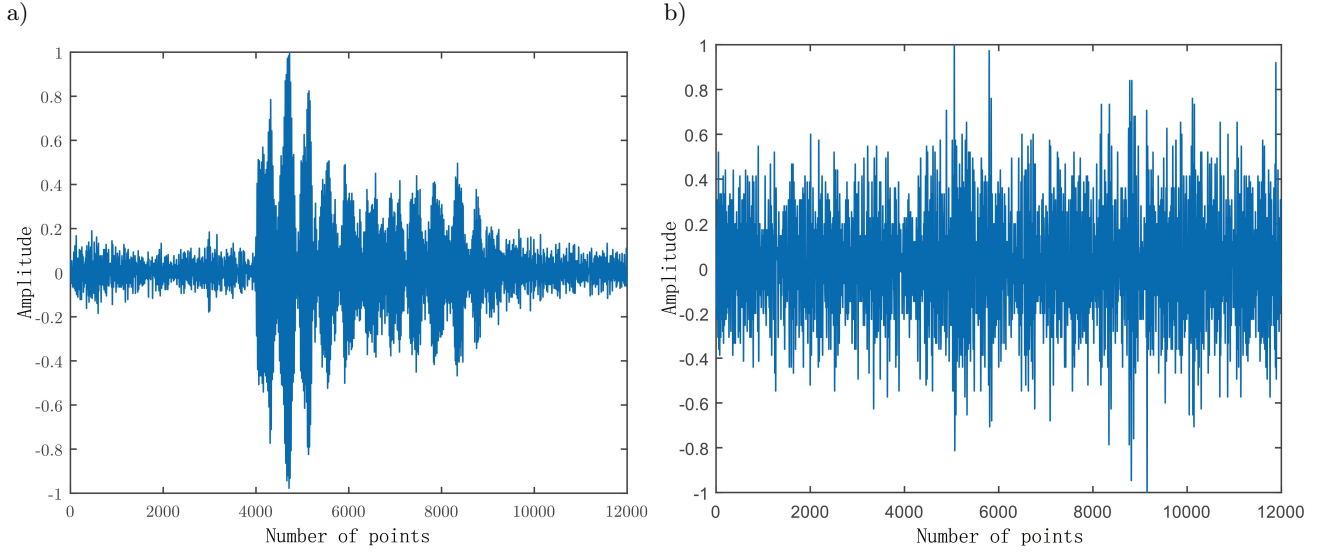
FIG. 6. Amplitude-normalized waveforms of target echo signal (a) and reverberation signal (b).
