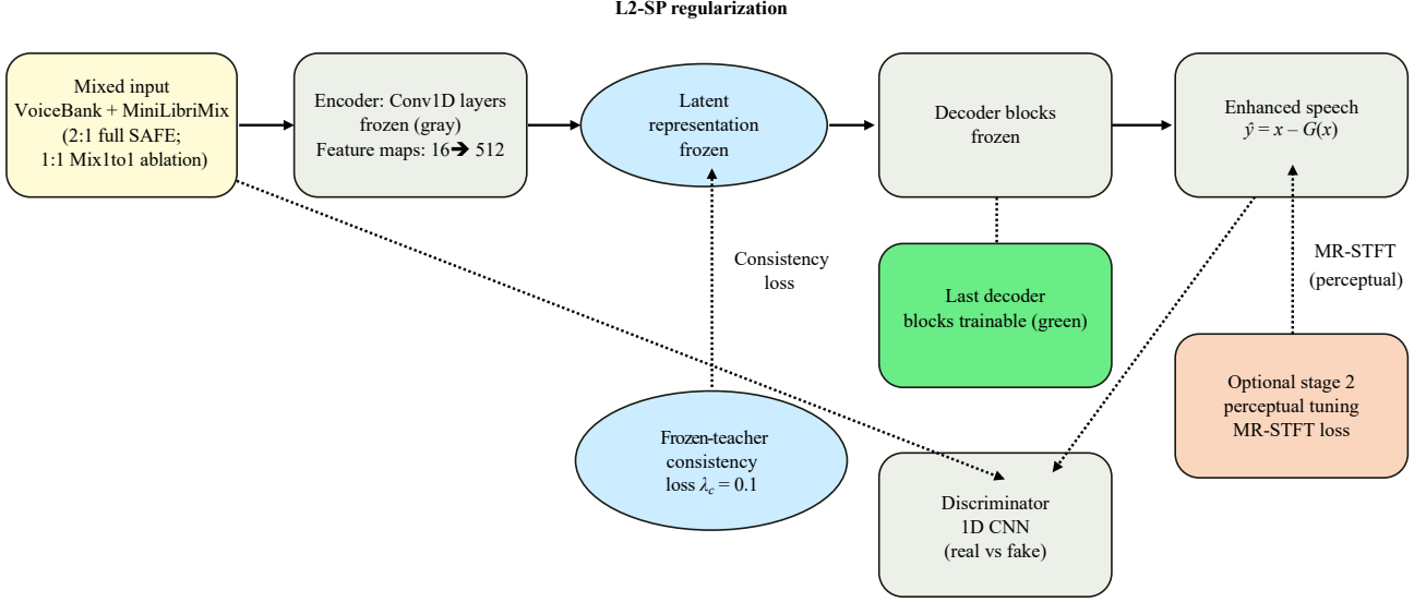
FIG. 3. SAFE adaptation architecture.
