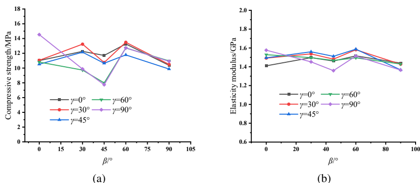
Fig. 9. Numerical simulation results of various \gamma values against changes in \beta ( a = b = 20 mm): (a) uniaxial compressive strength, (b) elasticity modulus
