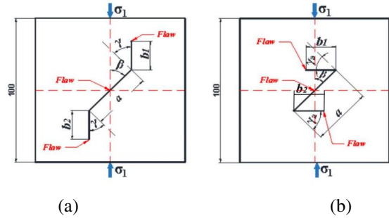
Fig. 1. Schematic diagram of uniaxial compression on specimens with Z-shaped fracture (Unit: mm): a) Type A, b) Type B
