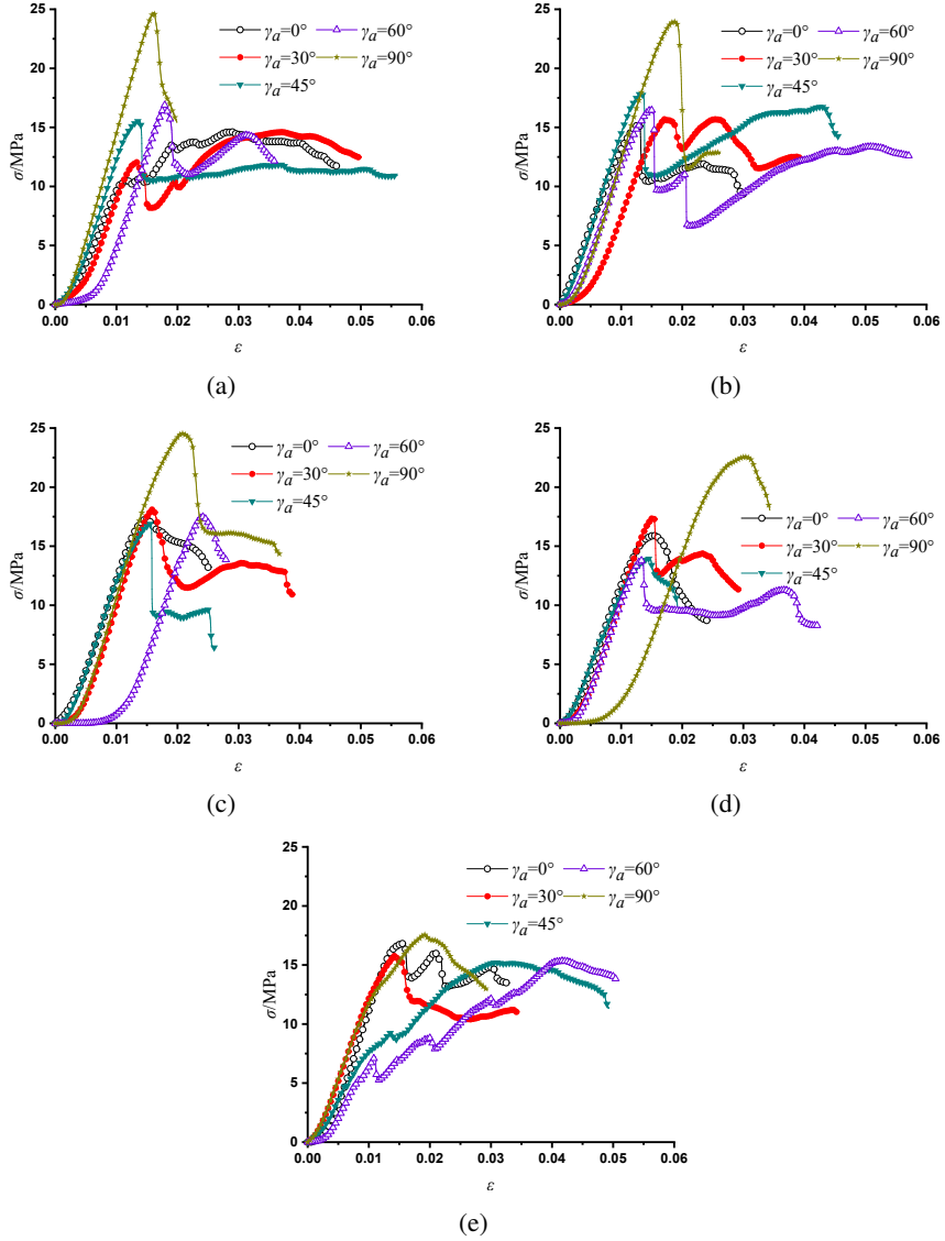
Fig. 3. Influence of \beta on the stress-strain curve of the specimen for each selected \gamma_a , a = b = 20 mm: : (a) \beta = 0^\circ , (b) \beta = 30^\circ , (c) \beta = 45^\circ , (d) \beta = 60^\circ , (e) \beta = 90^\circ
