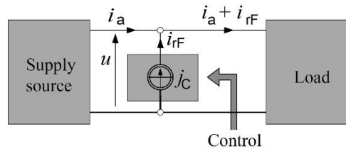
Fig. 3. A load with a controlled current source j(t)
