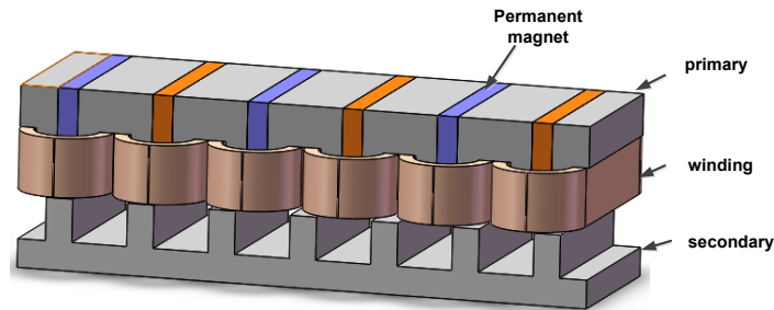
(a) PMFSLM 3D structure diagram
