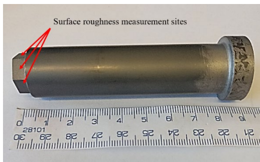
Fig. 14. Roughness measurement locations
