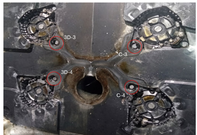
Fig. 2. Positions of the conventionally manufactured components C-3 and C-4 and the additively manufactured components 3D-3 and 3D-4 in the die-casting mould
