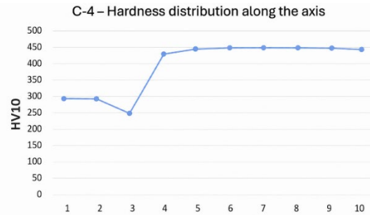
Fig. 19. Hardness development in component C-4
