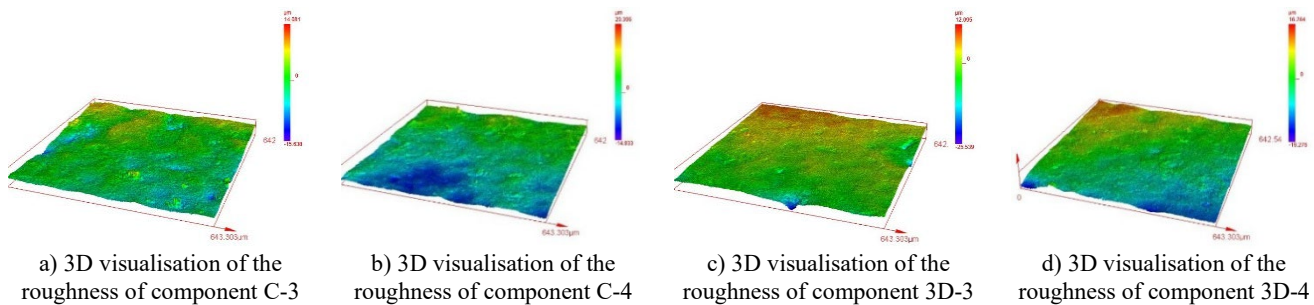
Fig. 16. Visualisation of component roughness
