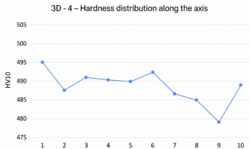
Fig. 21. Hardness development in component 3D-4
