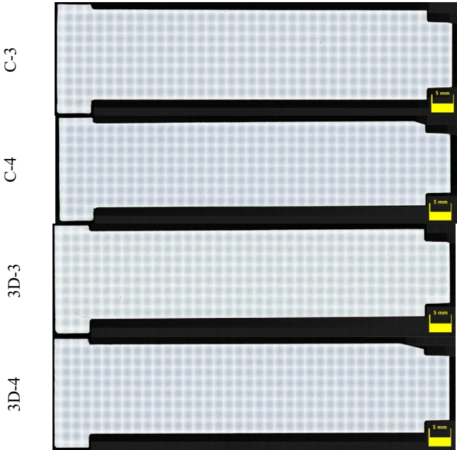
Fig. 13. Porosity distribution in conventionally and additively manufactured H13 components.
