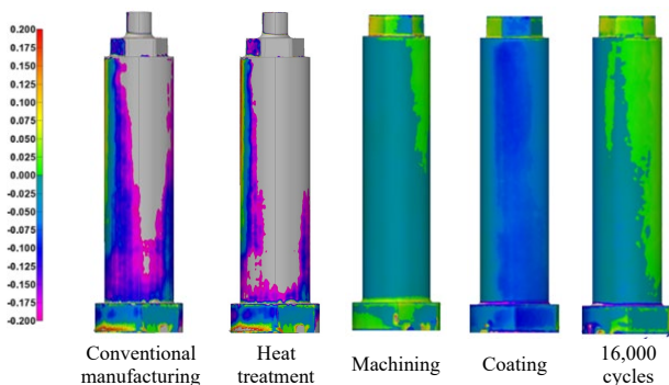
Fig. 7. First part of the technological process of component C-4
