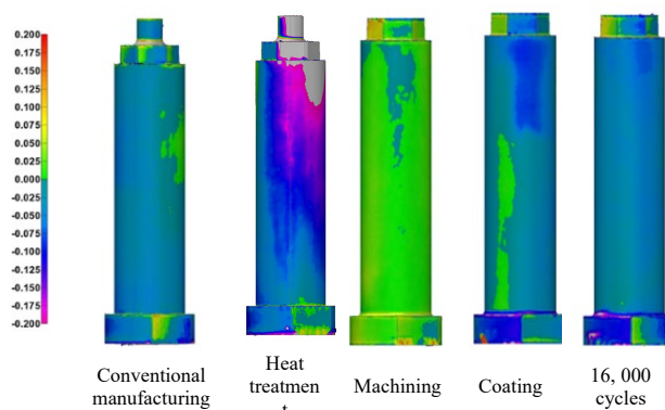
Fig. 5. First part of the technological process of component C-3
