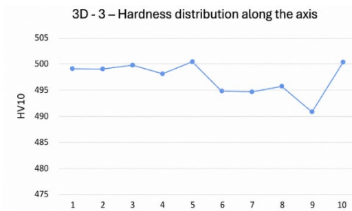
Fig. 20. Hardness development in component 3D-3
