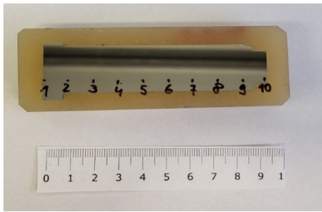
Fig. 17. View of the mounted and ground sample for hardness measurement
