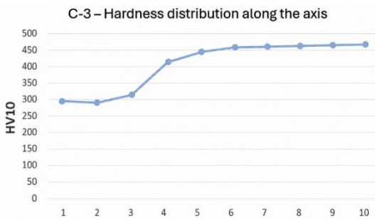
Fig. 18. Hardness development in component C-3
