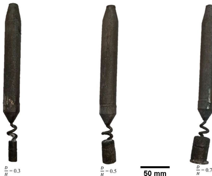
Fig. 3. Image of single crystal castings along with the grain selection system after separation from the central runner
