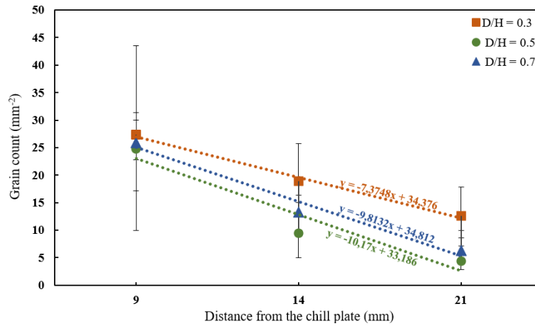
Fig. 18. Grain count per unit area as a function of distance from the chill plate for starter blocks with D/H ratios of 0.3, 0.5, and 0.7. The symbols represent the mean grain count, the error bars indicate the observed minimum-to-maximum range from six spatially separate measurements, and the dotted lines represent linear regression fits for the respective D/H ratios
