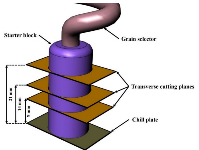
Fig. 16. Schematic illustration of the cross-section of the starter block at different distances from the chill plate
