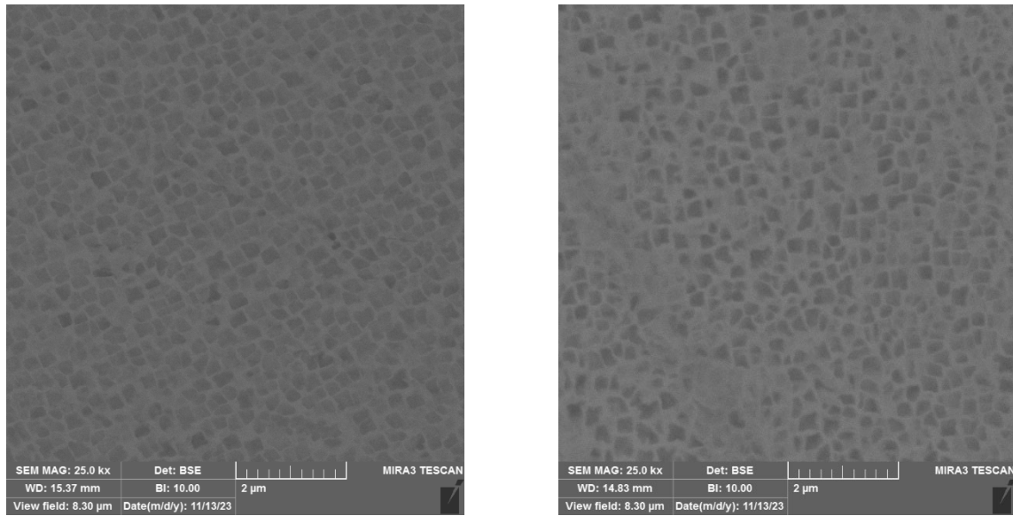
Fig. 15. SEM-BSE images of the primary dendrite core regions in single-crystal parts produced using starter blocks with diameter-to-height (D/H) ratios of (a) 0.3 and (b) 0.5
