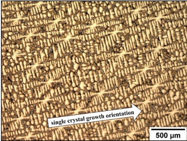
Fig. 13. Optical microscope image of the longitudinal section of single crystal part with starter block diameter-to-height ratio of 0.5
