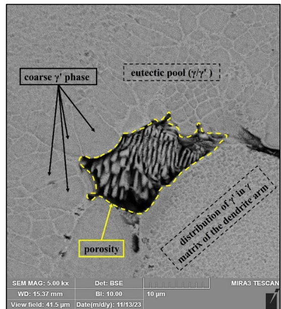
Fig. 9. SEM-BSE image of the interdendritic region of the single crystal casting with a starter block diameter-to-height ratio of 0.5, taken at a magnification of 5000 \times .
