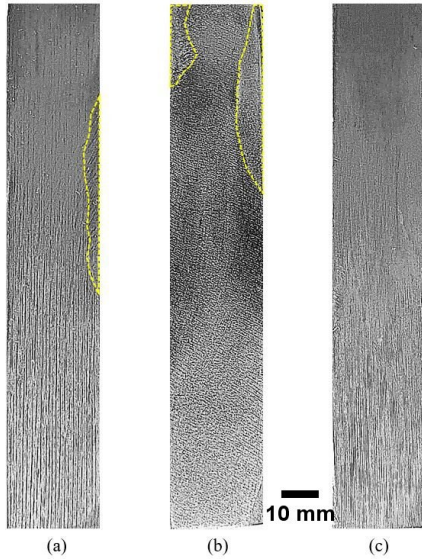
Fig. 5. Macroscopic image of etched longitudinal sections of single crystal castings with starter block diameter-to-height ratios of a) 0.3, b) 0.5, and c) 0.7, showing stray grains highlighted by dashed regions.
