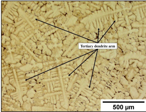
Fig. 19. Optical microscope image of the cross-section of starter block with diameter-to-height ratios of 0.7 at a distance of 30 mm from the chill plate
