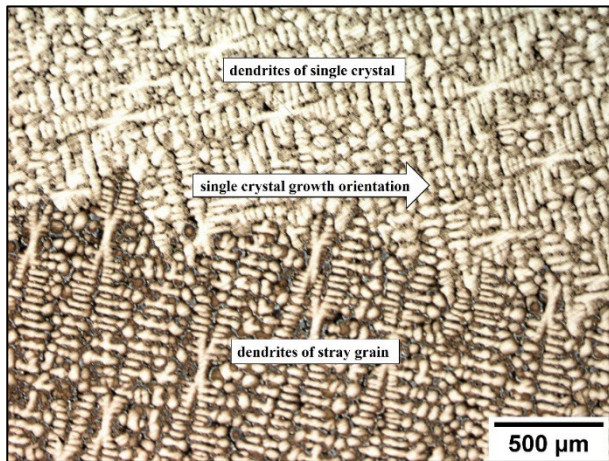
Fig. 7. Optical microscope image of the stray grain region in single crystal casting with starter block diameter-to-height ratio of 0.5.
