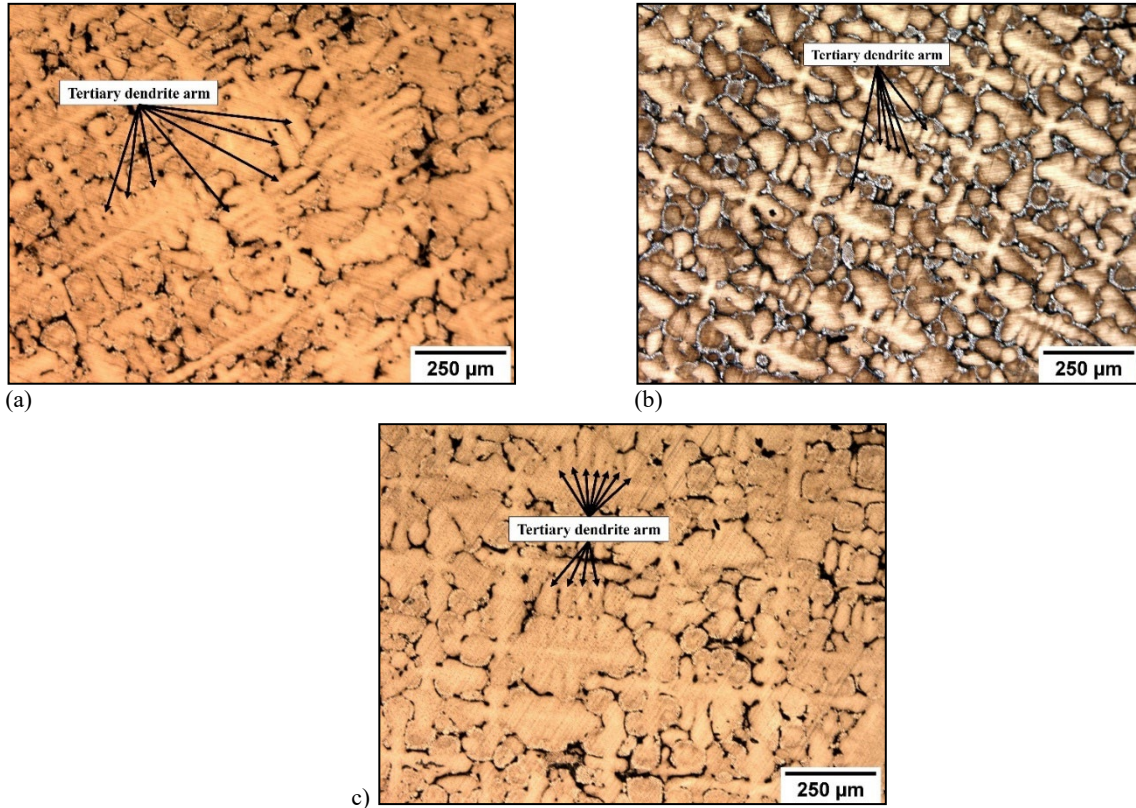
Fig. 10. Optical microscope images of the cross-sections of single crystal samples with starter block diameter-to-height ratios of a) 0.3, b) 0.5, and c) 0.7
