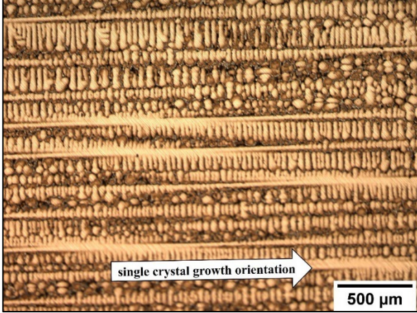
Fig. 12. Optical microscope image of the longitudinal section of single crystal part with starter block diameter-to-height ratio of 0.3
