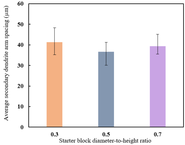
Fig. 14. Average secondary dendrite arm spacing in single crystal castings with diameter-to-height ratios of 0.3, 0.5, and 0.7
