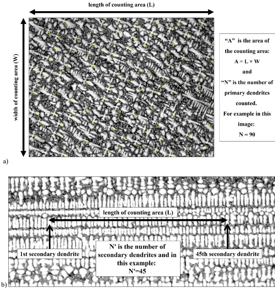
Fig. 2. Definition of variables in Equations a) 1 and b) 2
