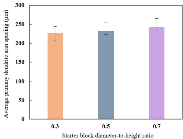
Fig. 11. Average primary dendrite arm spacing in single crystal castings with starter block diameter-to-height ratios of 0.3, 0.5, and 0.7
