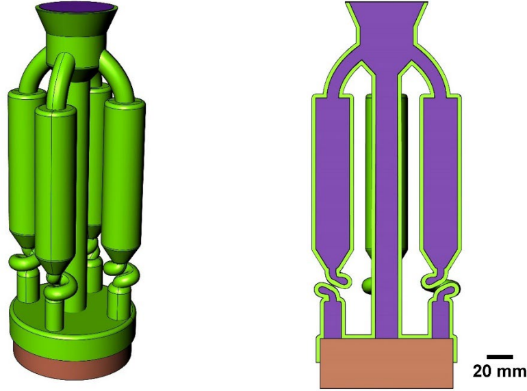
Fig. 1. Schematic diagram of the mold used in present study
