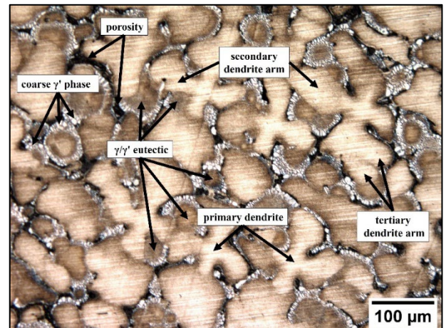
Fig. 8. Optical microscope image of the cross-section of the single crystal casting with a starter block diameter-to-height ratio of 0.5.
