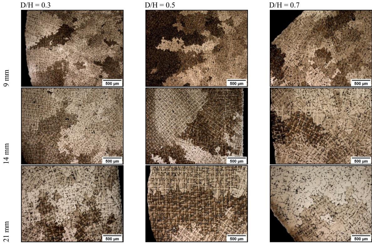
Fig. 17. Optical microscope images of cross-sections of starter blocks with different diameter-to-height ratios at distances of 9, 14, and 21 mm from the chill plate
