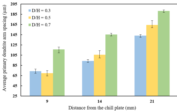
Fig. 20. Average primary dendrite arm spacing as a function of distance from the chill plate in starter blocks with different diameter-to-height ratios
