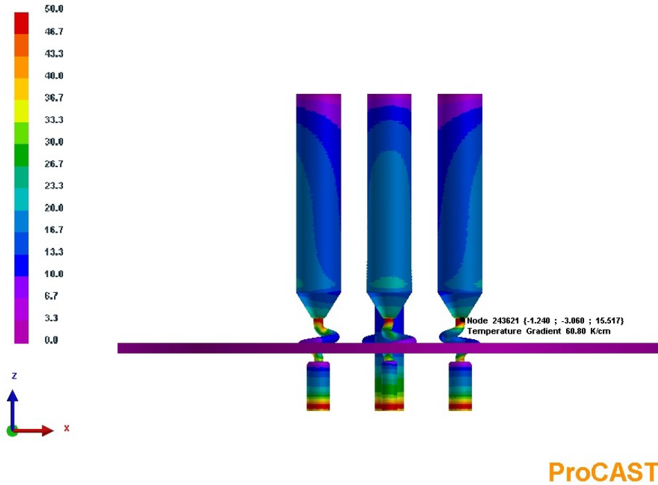
Fig. 6. ProCAST numerical simulation results showing the temperature gradient ( G ) distribution during the directional solidification of CMSX-4 castings with different starter block D/H ratios
