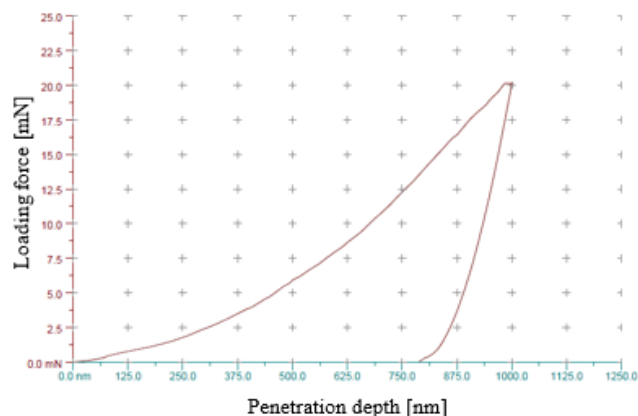
Fig. 8. Example indentation path of the indenter in the \beta(\alpha+\gamma) eutectic within the AZ91 alloy microstructure
