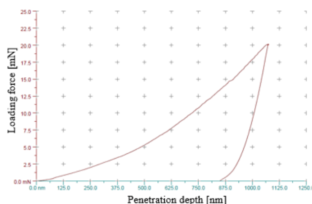
Fig. 6. Example indentation path of the indenter in the \alpha -Mg matrix within the AZ91 alloy microstructure
