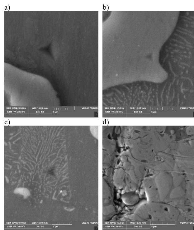
Rys. 5. Example of deep indentation in individual applications of the AZ91 microstructure: \alpha matrix (a), \gamma precipitate (b), \beta eutectic (c), and WCCoCr coating (d)
