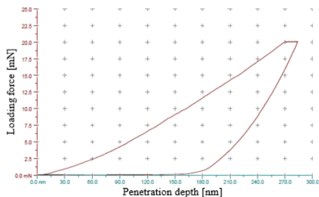
Fig. 9. Example indentation path of the indenter in a WCCoCr grain
