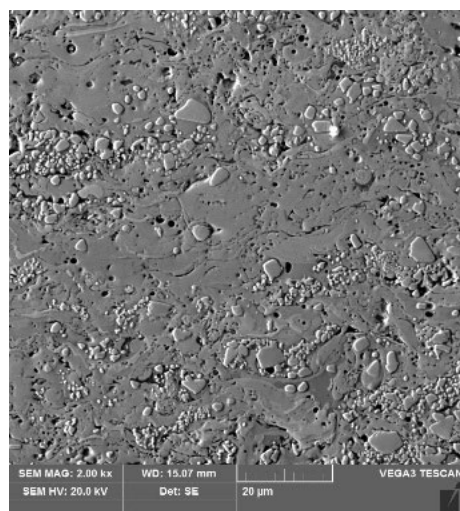
Fig. 4. Example view of the WCCoCr coating microstructure
