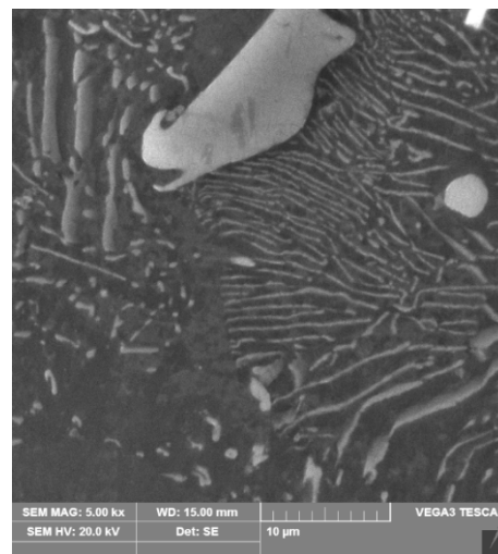
Fig. 1. Example microstructure of the AZ91 alloy (a) and high magnification of the eutectic \beta (b)
