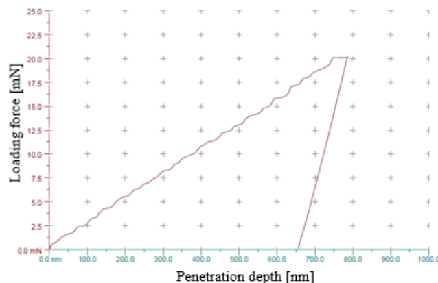
Fig. 7. Example indentation path of the indenter in the \gamma -Mg17(Al,Zn)12 phase within the AZ91 alloy microstructure
