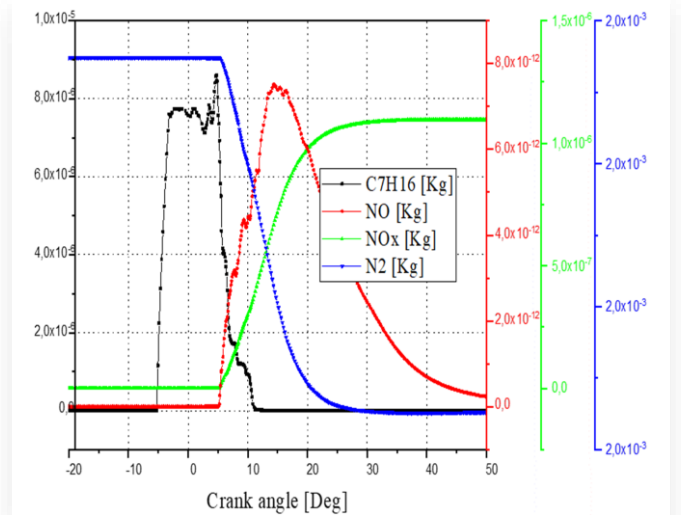
Fig. 10. Evolution of in-cylinder fuel mass and concentrations of NO, N_2 and NO_x .
