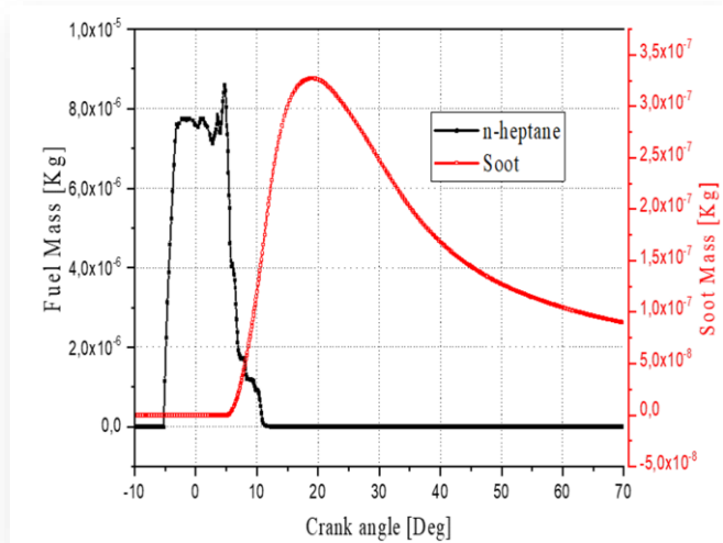
Fig. 8. Evolution of in-cylinder fuel mass and soot emission.
