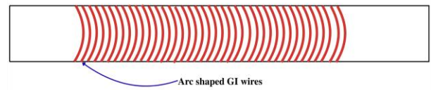
Fig. 23. Roughness geometry of arc-shaped parallel wires (drawn after [102]).
