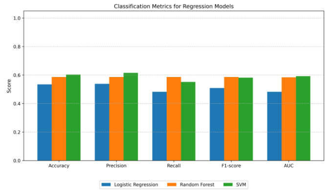
Fig.14. Classification metrics for classification models.
