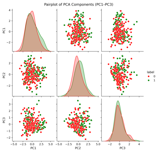
Fig.13. Pairplot of PCA Components.
