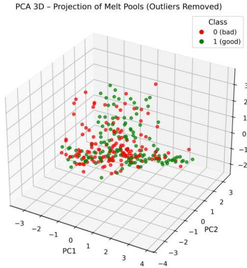
Fig.12. PCA projection for first three principal components.
