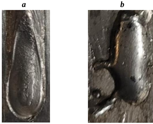
Fig.2. Weld pool images from the database, where: a) weld pool from acceptable welds and b) weld pool from unacceptable welds.
