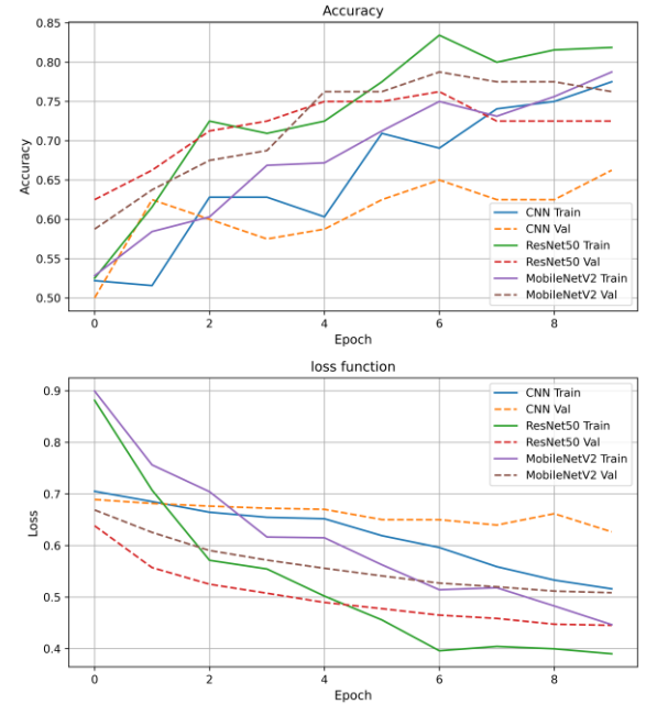
Fig.3. Learning curves and loss function curves for simple CNN model, ResNet50 and MobileNetV2.
