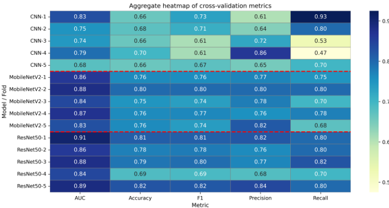
Fig.7. Cross-validation metrics for: CNN, ResNet50, and MobileNetV2.
