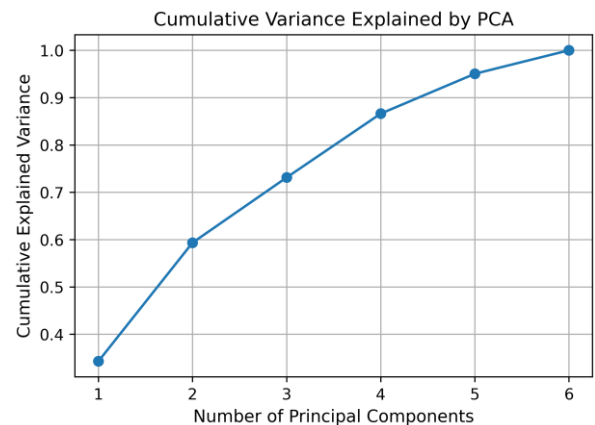
Fig.11. Cumulative Variance Explained by PCA.
