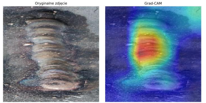
Fig.8. Grad-CAM visualizations for MobileNetV2 correct prediction.
