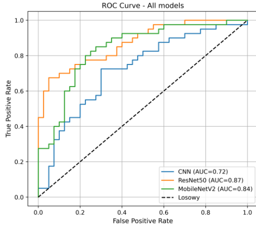
Fig.6. ROC curves for: CNN, ResNet50, and MobileNetV2.
