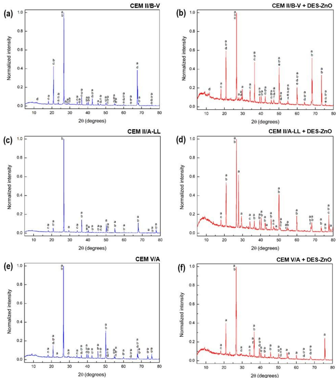
Fig. 5. XRD patterns of base cements: CEM II/B-V, CEM V/A, CEM II/A-LL and modified with 0.25% DES-ZnO. Peak labels corresponding to identified phases: a – alite, b – quartz, c – portlandite, d – gypsum, e – mullite, f – zincite. The intensities in the diffractograms were normalized to the maximum peak intensity
