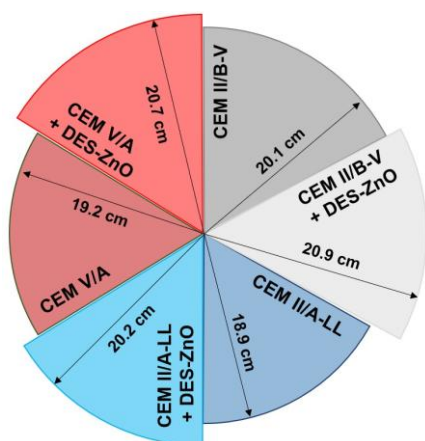
Fig. 1. Flow (cm) of cementitious mortars with and without DES-ZnO admixture
