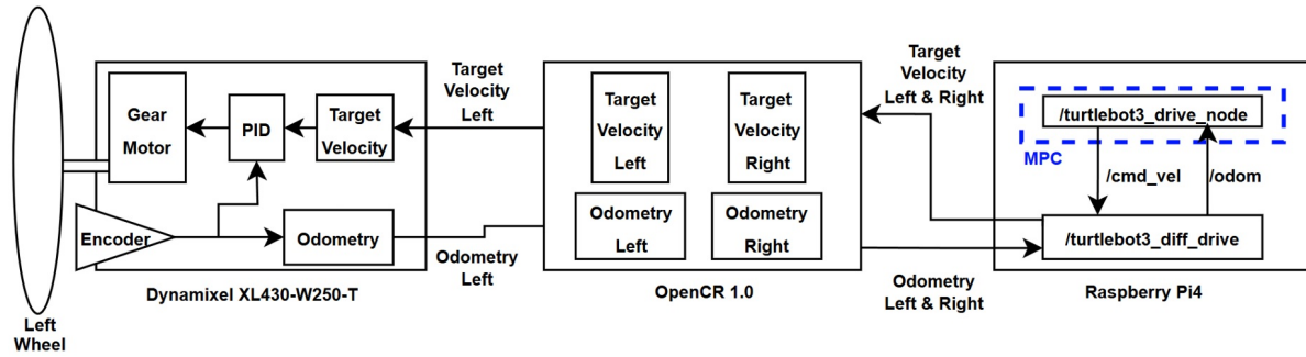
Fig. 7. TB3 motion system with implemented MPC controller
