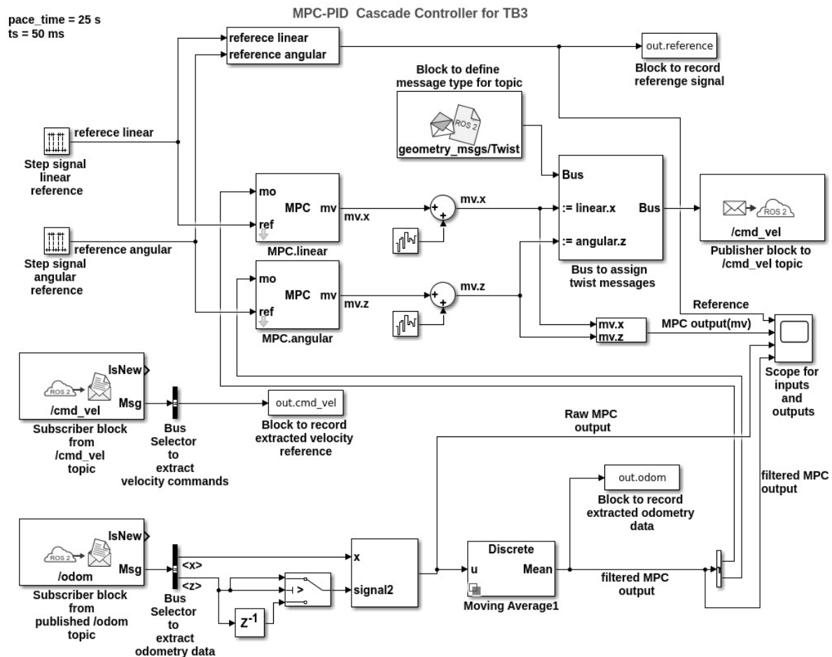
Fig. 8. Simulink model of proposed controller
