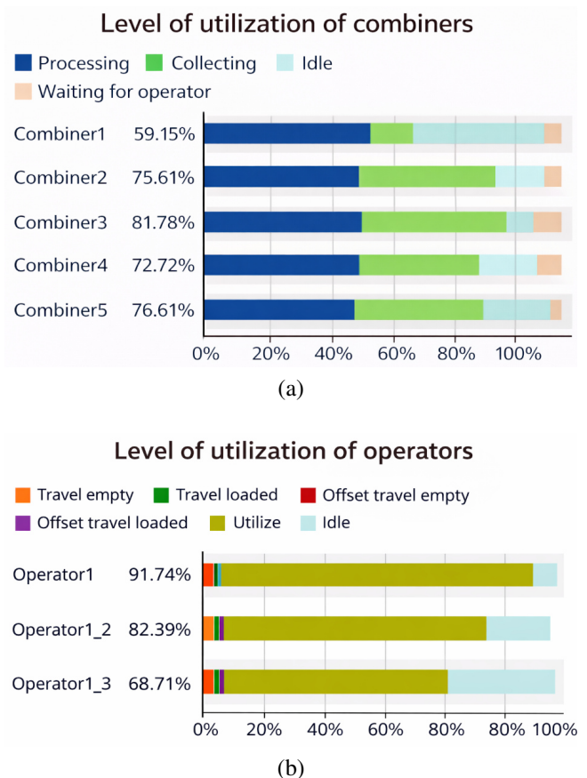
Fig. 15. Level of utilization in scenario S40 of: (a) combiners, (b) operators
