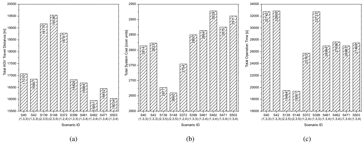
Fig. 11. Comparison of key performance indicators for selected Pareto-optimal solutions: (a) total travel distance, (b) total system cost, (c) total operation time (Variant II)
