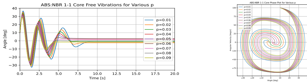
Fig. 7. Simulation results for ABS:NBR 1-1 core; ICs: \varphi_1(t) = 10 , \dot{\varphi}_1(t) = 100
