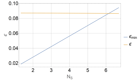
Fig. 10. The influence of external damping on the value of the parameter \varepsilon and on the value of the minimum of the unstable region \varepsilon_{\min} .
