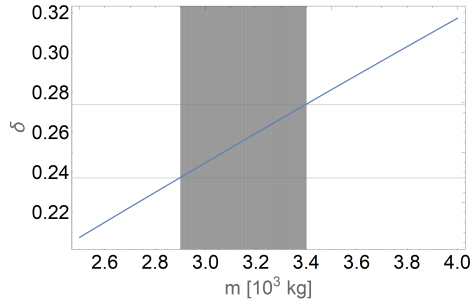
Fig. 6. Effect of load mass on the value of the \delta parameter, with the load mass range for unstable solutions indicated.
