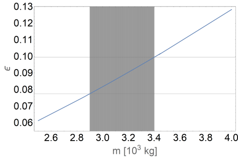
Fig. 7. Effect of load mass on the value of the \varepsilon parameter, with the load mass range for unstable solutions indicated.
