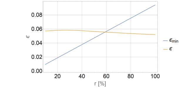
Fig. 13. The effect of internal, external, and structural damping on the value of parameter \epsilon and on the minimum value of the unstable region \epsilon_{\min} .
