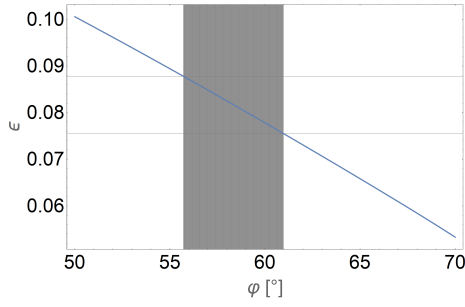
Fig. 5. Influence of the boom inclination angle on the value of the \varepsilon parameter, with the range of angles for unstable solutions marked.
