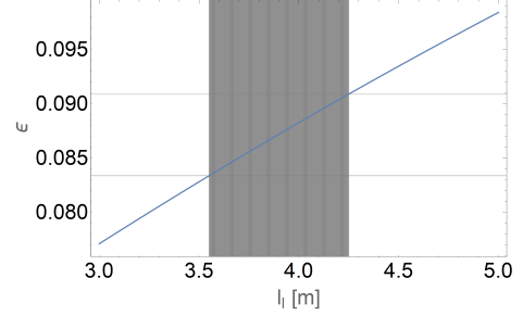
Fig. 9. Effect of rope length on the value of the \varepsilon parameter, with the rope length range for unstable solutions indicated.
