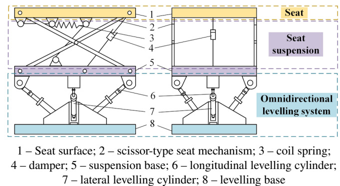
Fig. 1. Structure of the seat posture omnidirectional levelling system
