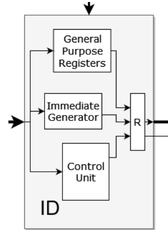
Fig. 6. The instruction decode module
