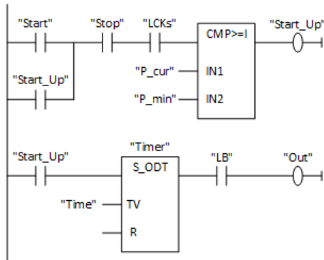
Fig. 2. LD control program
