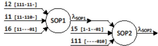
Fig.4. Technological representation of the analyzed function after creating two SOP blocks (SOP1 and SOP2)
