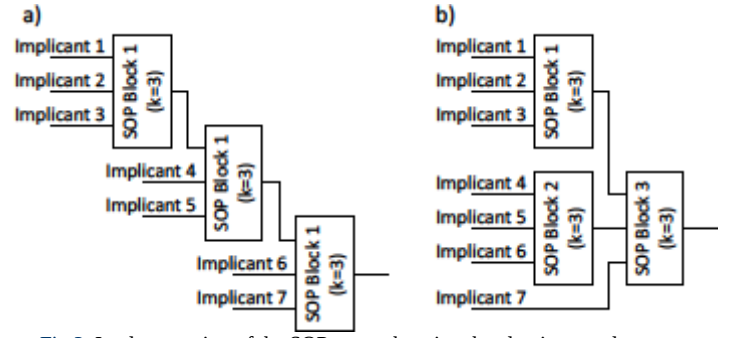
Fig.2. Implementation of the SOP network: using the classic cascade method (a) and the classic parallel method (b)
