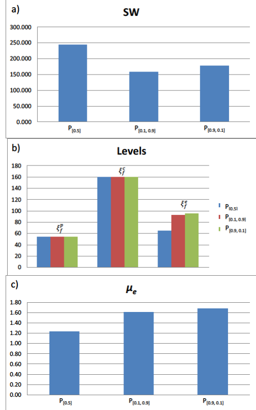
Fig.8. Obtained results of the SOP network mapping in 3-product blocks: total SW value (a), number of logical levels for the classic parallel method, cascade method and the proposed solution (b), average value of the \mu_e coefficient (c)
