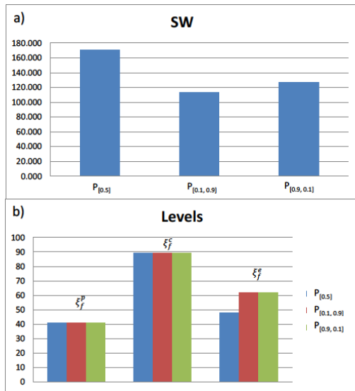
Fig.9. Obtained results of the SOP network mapping in 5-product blocks: total SW value (a), number of logical levels for the classic parallel method, cascade method and the proposed solution (b)
