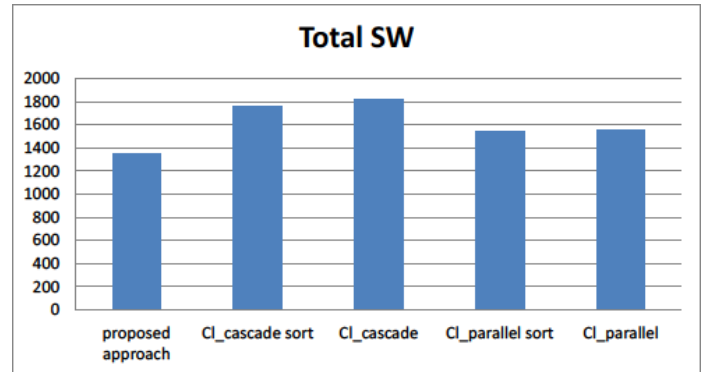
Fig.11. Comparison of SW for different mapping strategies in SOP networks
