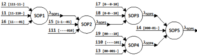
Fig.7. Network of SOP blocks representing an example function aimed at minimizing switching activity
