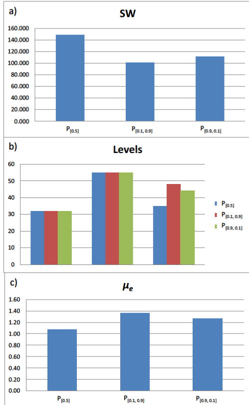
Fig.10. Obtained results of the SOP network mapping in 7-product blocks: total SW value (a), number of logical levels for the classic parallel method, cascade method and the proposed solution (b), average value of the \mu_e coefficient (c)
