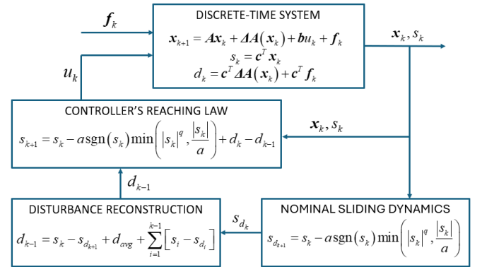
Fig. 1. Block diagram of the proposed control scheme.
