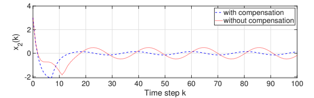
Fig. 3. Comparative performance of the state evolution.
