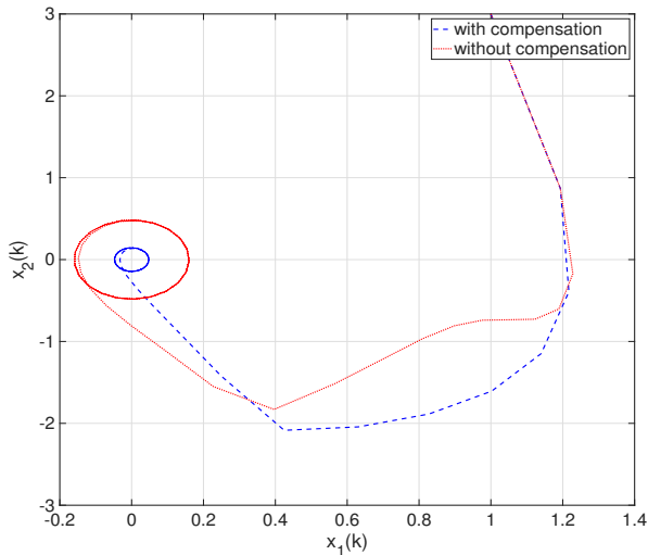
Fig. 4. Phase portrait of the state trajectories.
