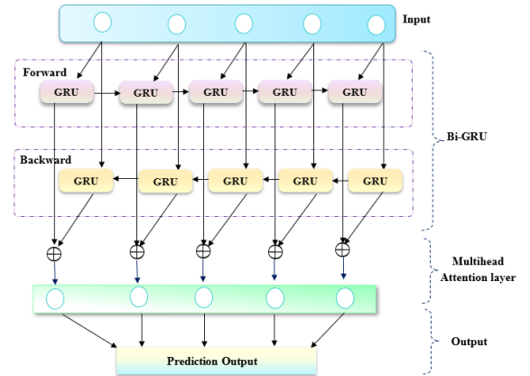
Fig.3. Architecture of MA-BiGRU
