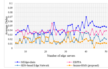
Fig.9. Average Delay Comparison
