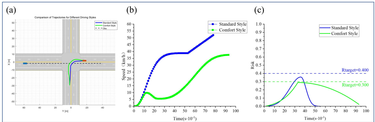
Fig. 10. Verification of driving style comparison: (a) trajectory comparison; (b) speed comparison; (c) risk comparison.
