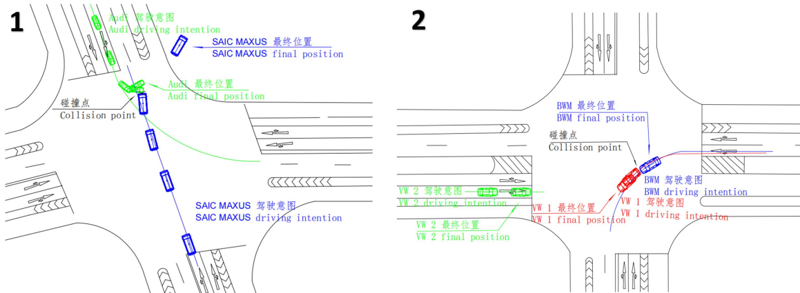
Fig. 1. Typical crash sequences reconstructed from NAIS data
