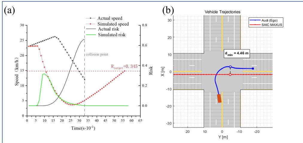
Fig. 8. Collision avoidance performance in Case 1.(a) Comparison of speed and risk profiles. The proposed method initiates early braking upon risk detection ( t \approx 0.8 \text{ s} ), preventing the collision occurred in the original case.(b) Vehicle trajectories. The ego vehicle yields to the obstacle, maintaining a safe clearance with d_{\text{min}} = 4.46 \text{ m} .
