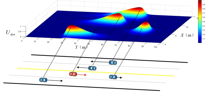
Fig. 5. DRF intensity distribution in complex traffic with relative motion to the ego vehicle.
