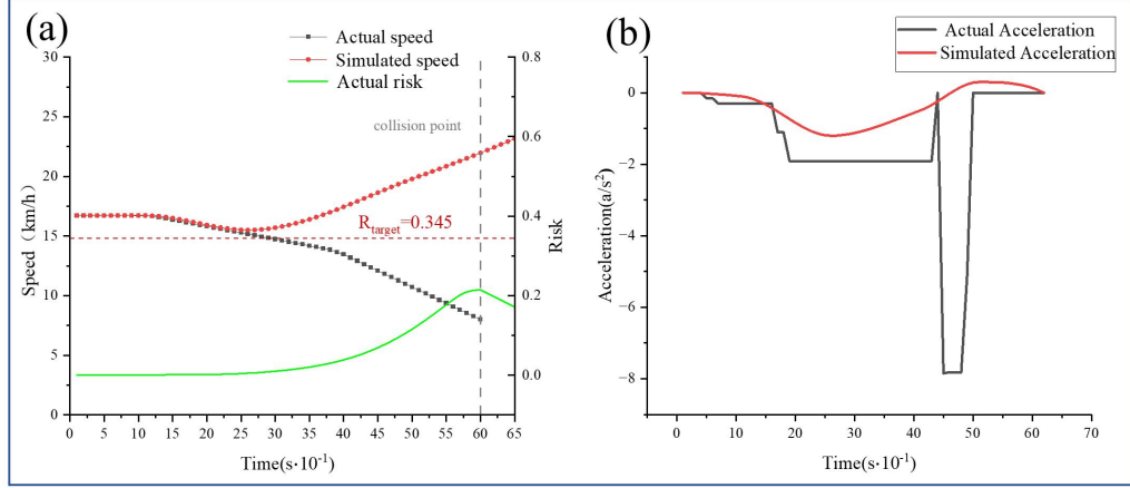
Fig. 9. Performance analysis in Case 2. (a) Decision-making process. The perceived risk remains below the target threshold ( R_{\text{target}}=0.345 ), allowing the ego vehicle to proceed smoothly without unnecessary hesitation. (b) Following vehicle response. The proposed method results in smooth deceleration, eliminating the emergency braking maneuver ( -7.85 \text{ m/s}^2 ) observed in the original crash case.
