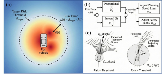
Fig. 7. Schematic of the Risk Homeostasis-based feedback mechanism. (a) Risk field intensity distribution and definition of risk error; (b) Structure of the PI controller for parameter adaptation; (c) Illustration of adaptive trajectory planning constraints (speed limit v_{lim} and safety buffer D_{buf} ) under different risk levels.
