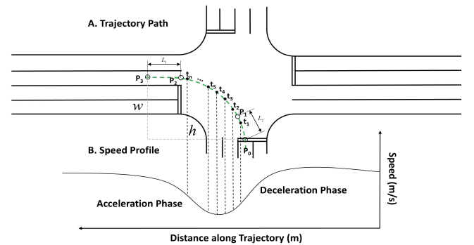
Fig. 2. Schematic of global reference trajectory planning.
