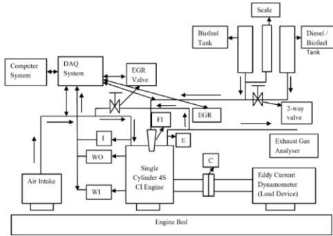
FI-Fuel Injector, I-Intake Valve, E-Exhaust Valve, C-Coupling, WO-Water Outlet, WI-Water Inlet (a)
