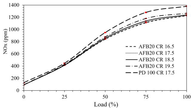
Fig. 10. Variation of NO x emissions with brake power for the AFB20 blend at different compression ratios. Error bars represent \pm expanded uncertainty (Table 5).
