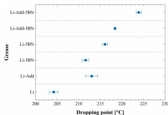
Fig.2. Dropping point of greases
