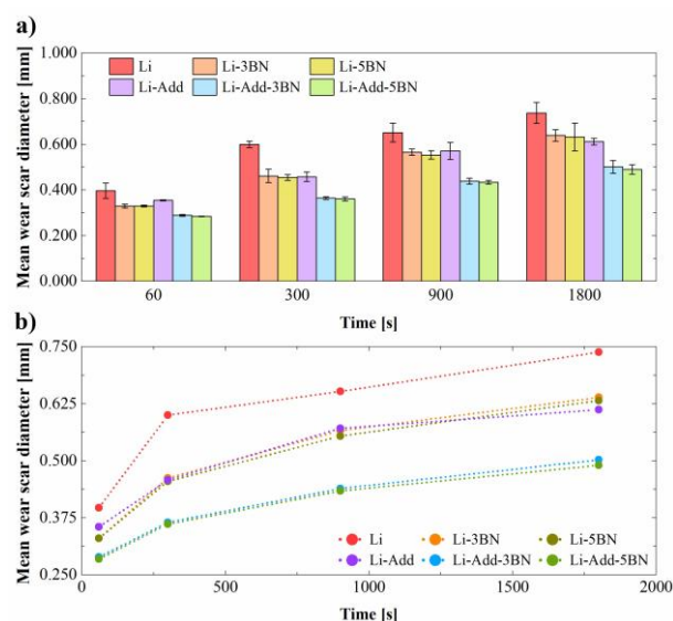
Fig.4. Tribological tests results: a) mean wear scar diameter after different test duration, b) changes in wear scar diameter as a function of test duration
