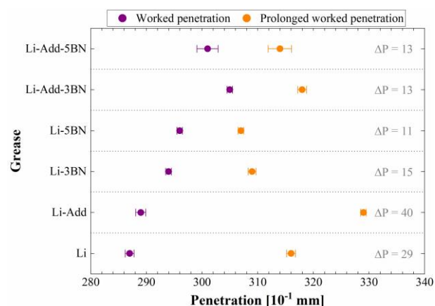
Fig.3. Penetration values and mechanical stability of greases
