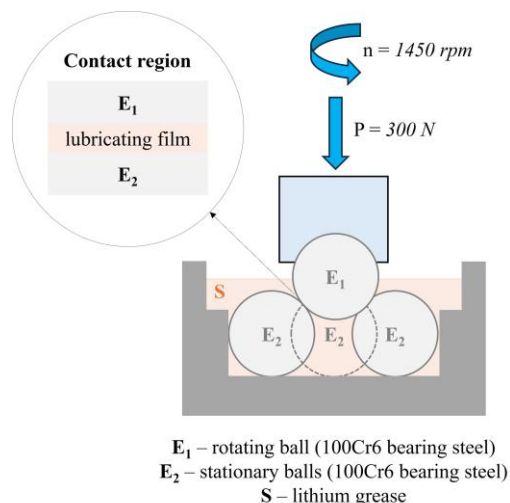
Fig.1. Schematic representation of the tribological system in a four-ball apparatus
