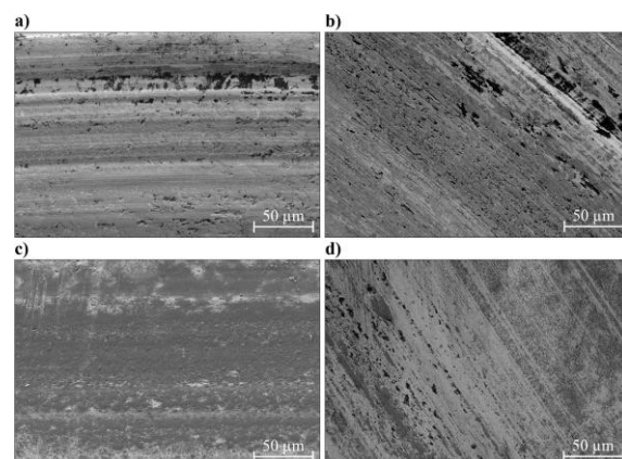
Fig.5. Wear scars surfaces: a) Li, b) Li-Add, c) Li-5BN, d) Li-Add-5BN
