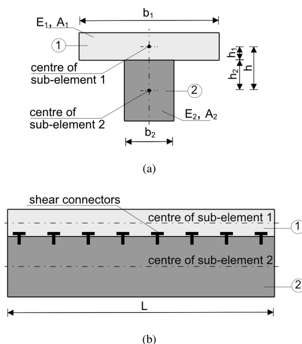
Fig. 1. Geometry of (a) the cross-section and (b) the longitudinal section of a two-layer element
