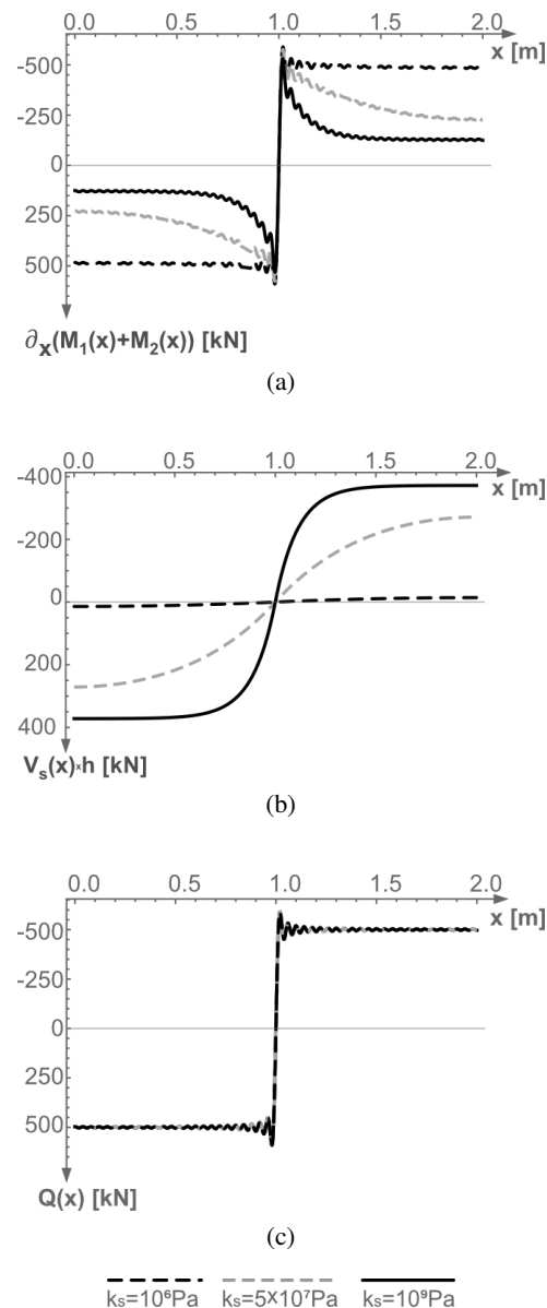
Fig. 6. Shear forces: (a) component \frac{dM_B(x)}{dx} , (b) component V_s(x) \cdot h , (c) shear forces Q(x)
