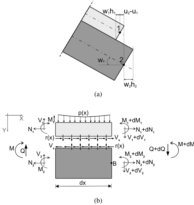
Fig. 2. (a) Mutual displacements of the components of a two-layer beam; (b) Internal forces in the cross-section of the two-layer beam and at the interface of the component layers along section dx
