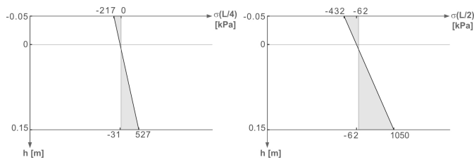
Fig. 8. Normal stress diagram in cross-section x = L/4 (on the left) and x = L/2 (on the right) when k_s = 10^{14} Pa
