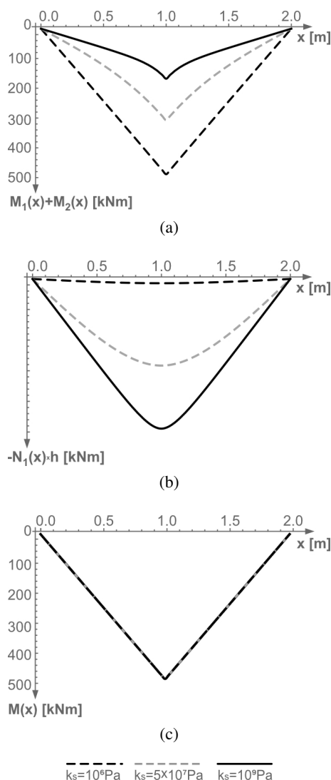
Fig. 5. Bending moments: (a) component M_1(x) + M_2(x) , (b) component -N_1(x) \cdot h , (c) diagram of bending moments M(x)
