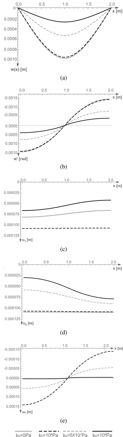
Fig. 4. Dependence between: (a) displacement w(x) , (b) rotation angle w'(x) , (c) displacement u_1(x) , (d) displacement u_2(x) , (e) the mutual slip between layers u_s and the value of the k_s parameter
