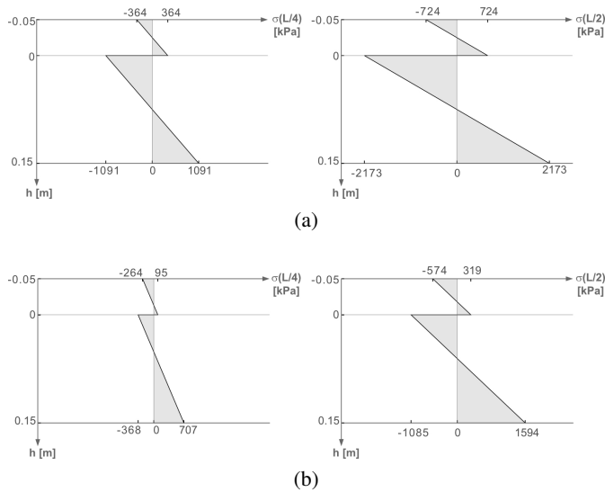
Fig. 7. Normal stress diagram in cross-section x = L/4 (on the left) and x = L/2 (on the right) when (a) k_s = 0 Pa, (b) k_s = 5 \cdot 10^7 Pa
