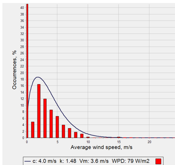
Fig. 5. Weibull distribution model for Zhambyl region (latitude 43.546411, longitude 75.270432)
