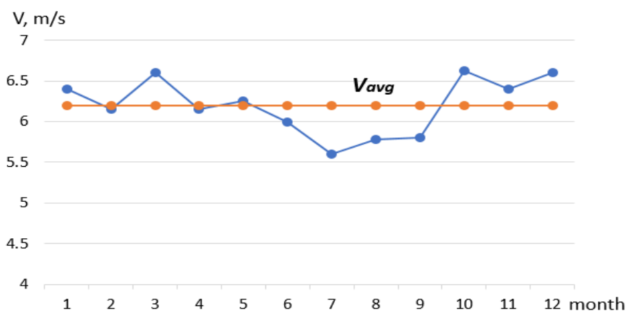
Fig. 2. Annual changes in wind speed Source: compiled by the authors based on United Nations Development Programme (UNDP) Kazakhstan (2011)
