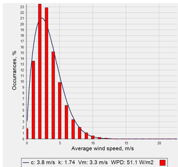
Fig. 4. Weibull distribution model for the Talgar region (latitude 44.219675, longitude 77.132173)
