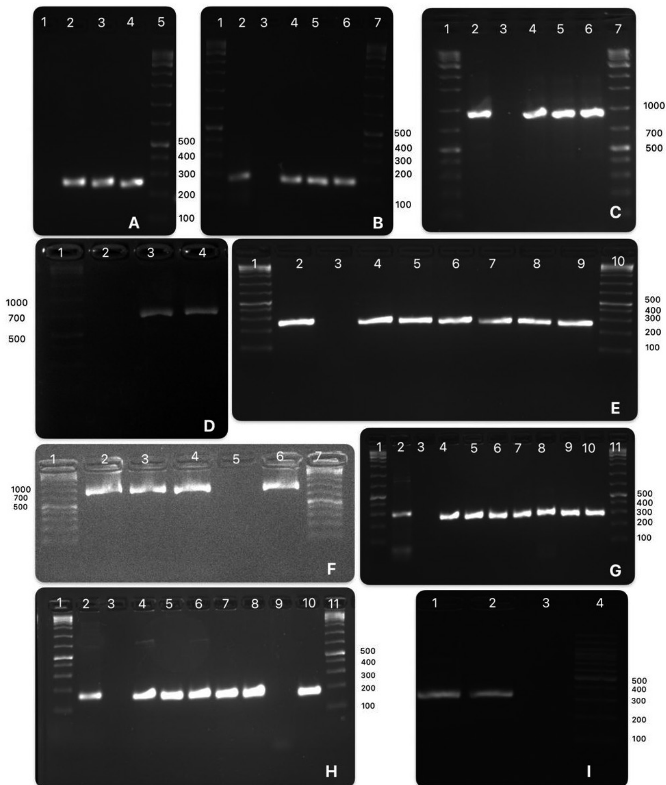
Fig. 2. Agarose gel electrophoresis images of PCR amplicons for the pav , PsaA , LP1 , LP2 , LP3 , LP4 , AC1 , AC2 , and AF genes, shown sequentially. In each image, M denotes the molecular size marker (GRS Universal Ladder, GRiSP), P the positive control, N the negative control, and lanes 1-10 the sample isolates.
