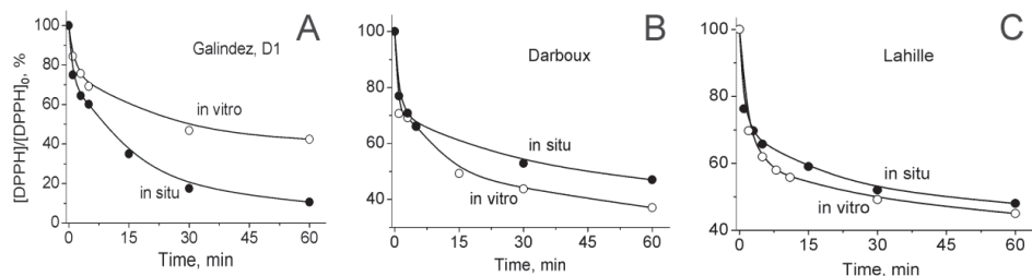
Fig. 13. Inhibition of DPPH radicals by the extracts of Deschampsia antarctica wild plants sampled from the maritime Antarctic and plants cultivated in vitro . (after Ivannikov et al. 2021a).
