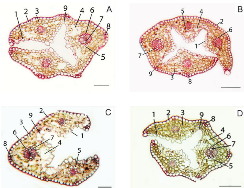
Fig. 5. Cross-sections of the leaves of Deschampsia antarctica in vitro plants of four different genotypes: A – W1; B – S22; C – DAR12; D – Y66. 1 – adaxial epidermis, 2 – abaxial epidermis, 3 – mesophyll, 4 – intercellular space, 5 – exterior sheath of the vascular bundle, 6 – interior bundle sheath, 7 – metaxylem, 8 – sclerenchyma, 9 – motor cells. Scale bars = 100 \mu m (after Nuzhyna et al. 2021).
