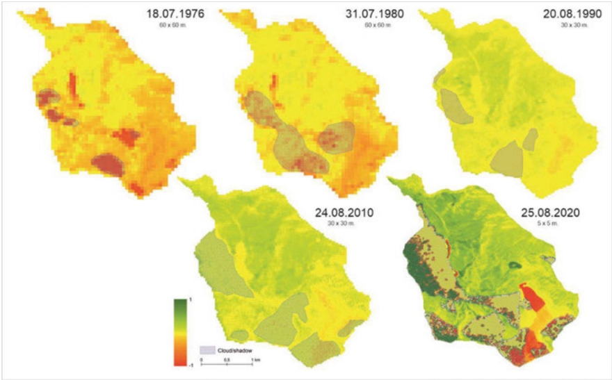
Fig. 9. The Normalized Difference Vegetation Index for the years 1976, 1980, 1990, 2010 and 2020 with marked cloud/shadow coverage excluded from the analysis in the Bratteggelva catchment.
