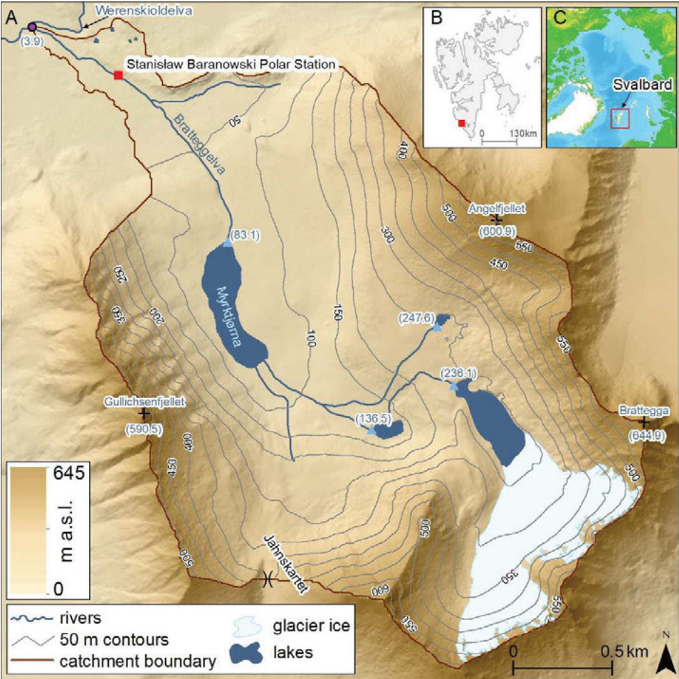
Fig. 1. Overview map of the study area: A - the Bratteggelva catchment, modified from ArcticDEM (Porter et al. 2018), contours based on digital elevation model; B - map of Svalbard, location of study area indicated by red square (Modified from Norwegian Polar Institute 2014a); C - polar projection map of the Arctic Ocean (data provided by Arctic-SDI geoportal).
