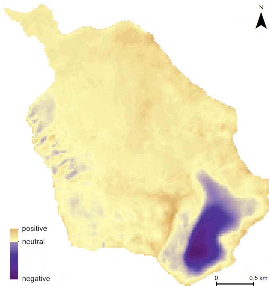
Fig. 8. Elevation change between years 1936 and 2011, based on 20x20 m resolution DEMs from 1936 (Geyman et al. 2022b) and 2011 (Norwegian Polar Institute 2014b).
