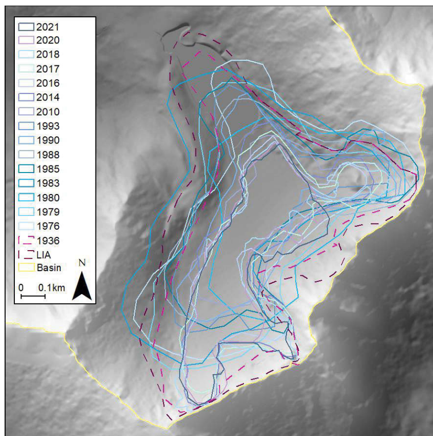
Fig. 10. Brattegggreen areal change since 1975. Based on satellite images for years 1976–2017 Landsat, source: www.earthexplorer.usgs.gov/ ; 2018–2021 Sentinel, source: https://apps.sentinel-hub.com/eo-browser/ and based on Geyman et al. (2022b) for year 1936. Some shifts are caused by offsets of satellite images and their lower resolution.
