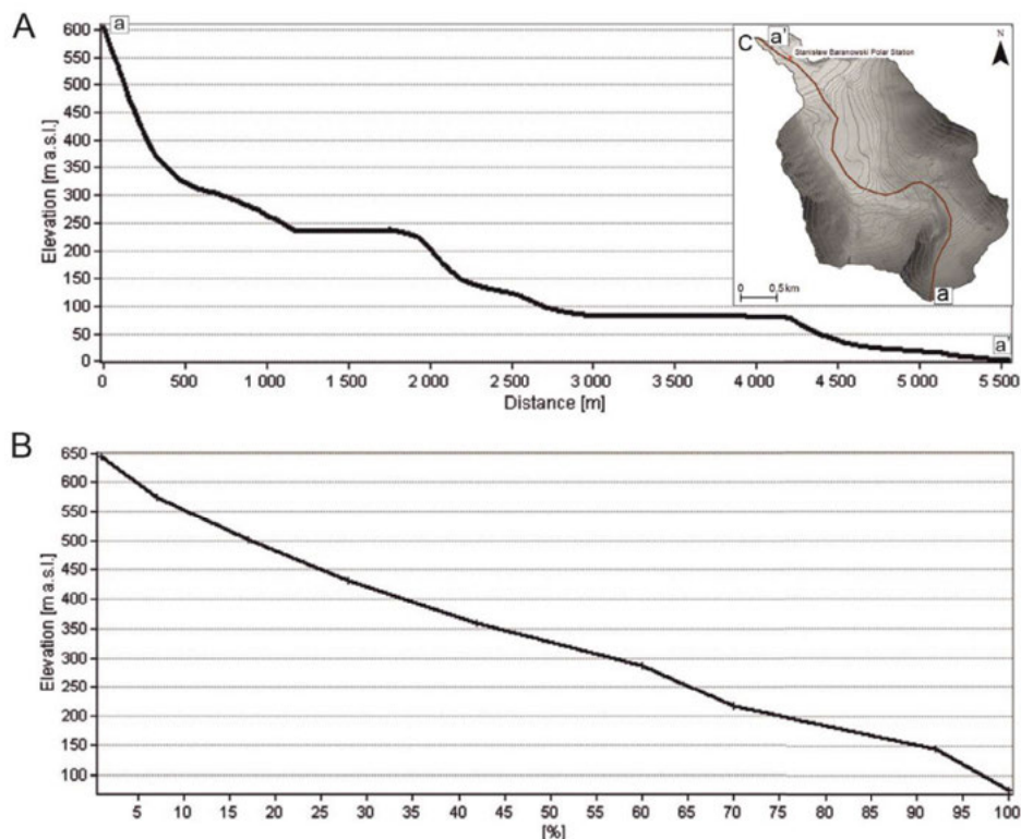
Fig. 3. Longitudinal profile (A), map showing location of the profile (C) and hypsometric curve (B) of the Bratteggelva catchment, based on digital elevation model.
