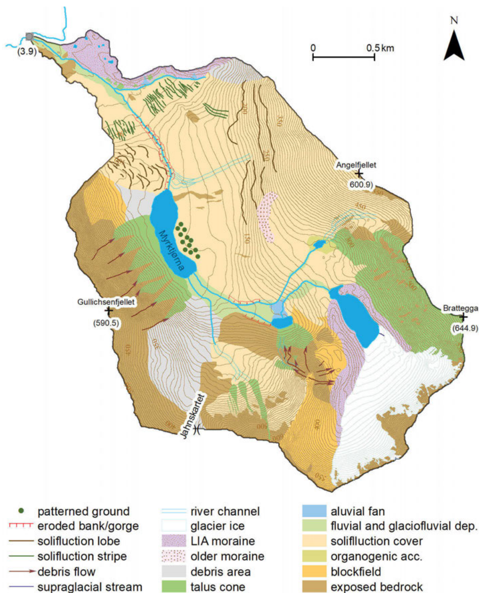
Fig. 4. Geomorphological map of the Bratteggeva catchment.
