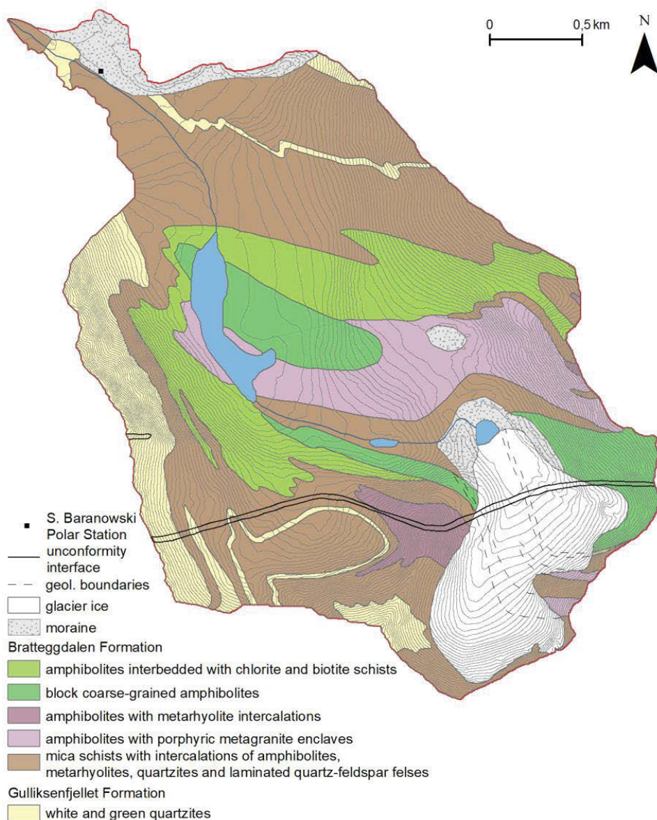
Fig. 2. Geological map of the study area modified from Czerny et al. (1993). Note different extent of the glacier and lakes as compared to Fig. 1, which is due to considerably earlier time of mapping.
