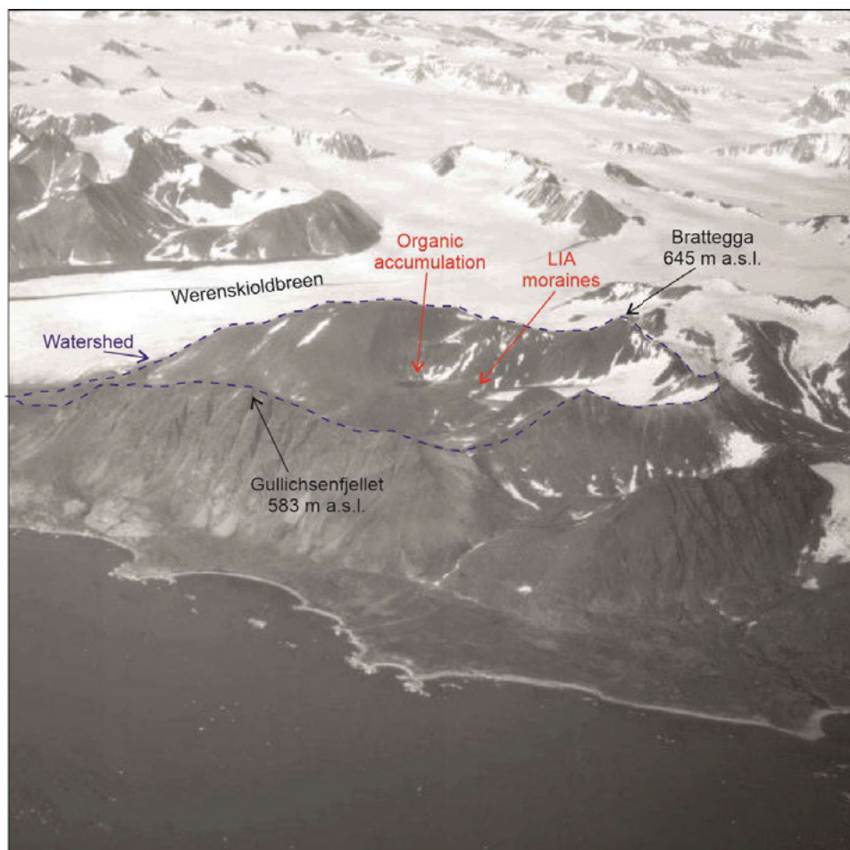
Fig. 11. Aerial photo of the Bratteggelva catchment from 1936, modified after Geyman et al. (2022b).
