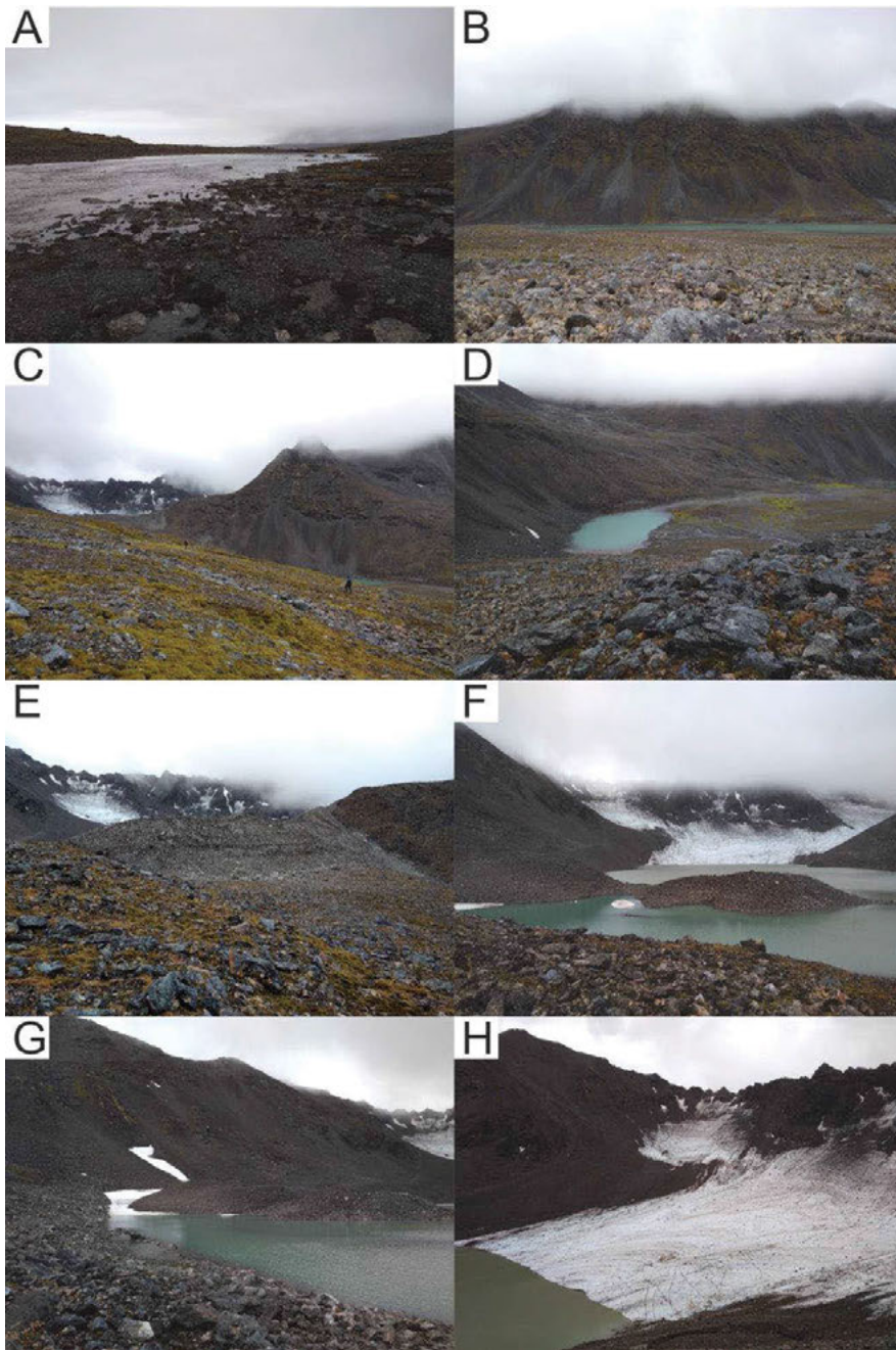
Fig. 7. Photographs from the fieldwork in 2018: A - the Myrktjørna lake; B - talus cones; C - view from Anglefjellet slope of the upper part of the Bratteggelva catchment; D - view of the middle lake; E - the LIA moraine of Bratteggreen; F - view of the Bratteggreen with the glacial lake and moraines; G - view of the Eastern side of the Bratteggreen moraines and the slopes above Bratteggreen; H - Bratteggreen in 2018.
