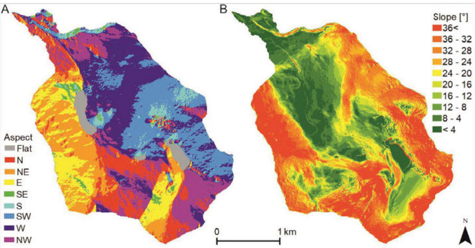
Fig. 6. Aspect (A) and slope (B) in the Bratteggelva catchment, based on digital elevation model.
