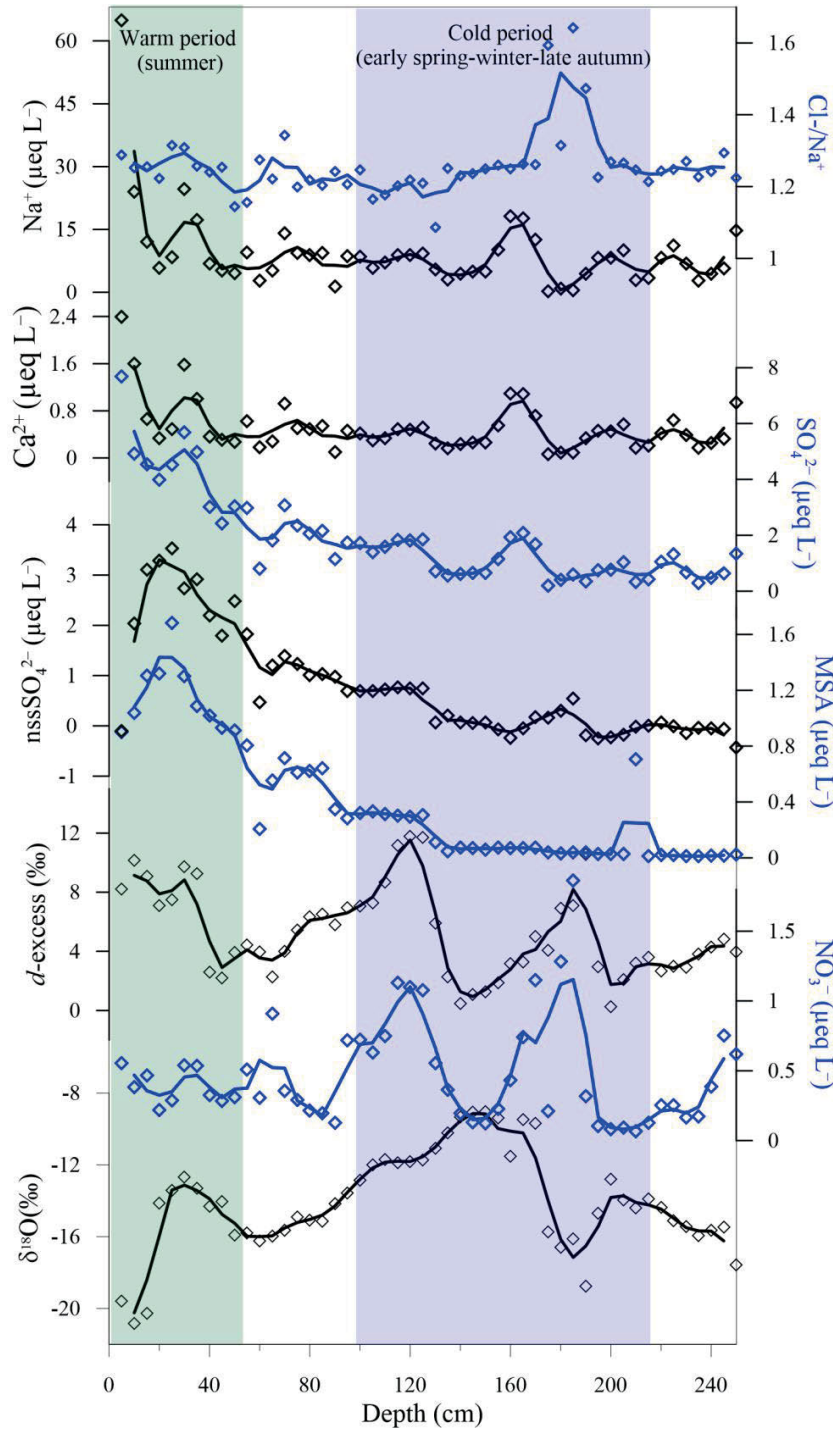
Fig. 4. Depth vs. \delta^{18}\text{O} , d\text{-excess} , \text{NO}_3^- , \text{MSA} , \text{nssSO}_4^{2-} , \text{SO}_4^{2-} , \text{Ca}^{2+} , \text{Na}^+ , and \text{Cl}^-/\text{Na}^+ . Thick lines represent the three-point running average profiles.
