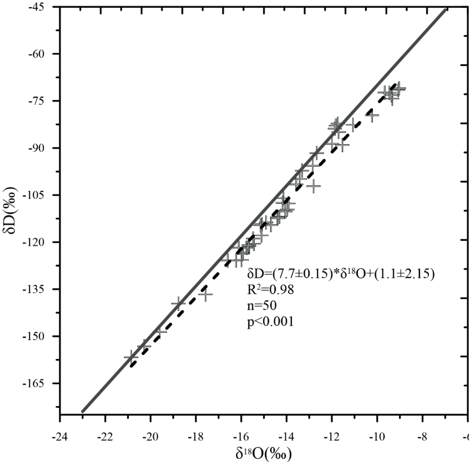
Fig. 3. \delta^{18}\text{O} - \delta\text{D} diagram of the snow-pit marked as the dashed line with the Global Meteoric Water Line of Craig (1961) marked as the solid line.
