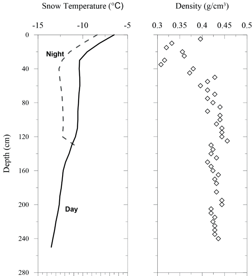
Fig. 2. Vertical profiles of snow temperature and density in the Moore Dome snow-pit.
