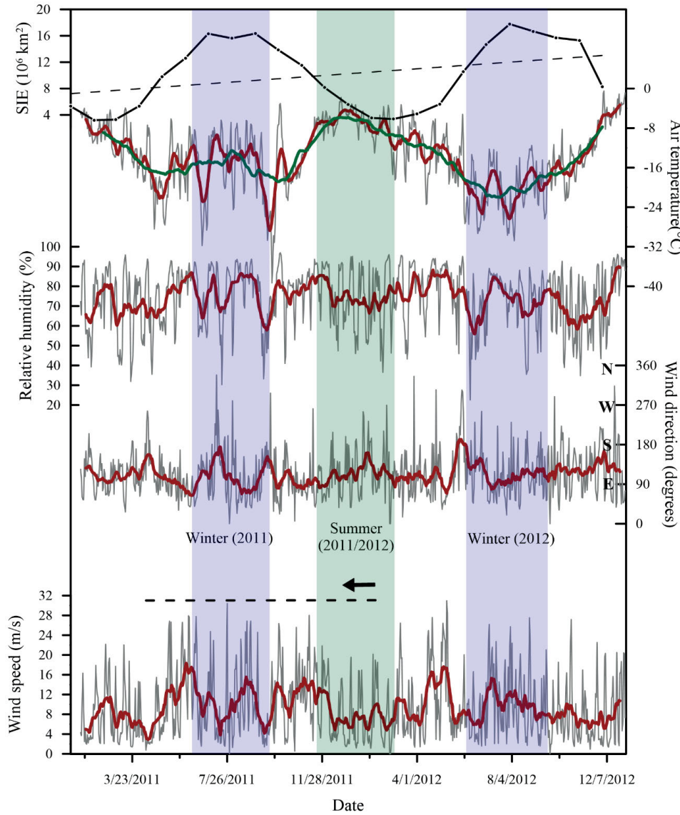
Fig. 5. Daily mean (grey line) and 15-point running averaged (red line) meteorological data between January 2011 to December 2012 in Bear Peninsula automatic weather station with monthly mean sea ice extent data. The green line is 60 day-average air temperature. Purple and green shading indicate winter and summer seasons, respectively. The horizontal dashed line and arrow indicate the period covered in the Moore Dome snow-pit. We note that the top layers of the snow-pit corresponding to the summer 2011/2012 was relatively clear, however bottom depth is roughly assumed to extend to winter 2011.
