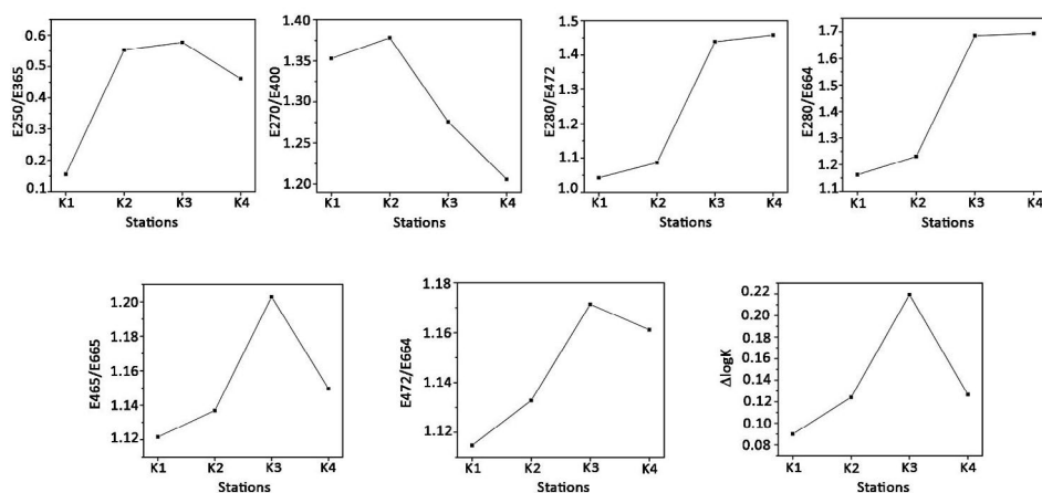
Fig. 2. UV-visible spectroscopic ratios of various humic acids isolated from Krossfjorden sediments.
