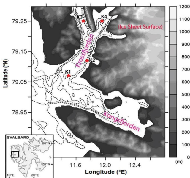
Fig. 1. Map of the Krossfjorden from the GEBCO 2020 data. The dashed contour lines represent the bathymetry. The red symbol represents the station locations. The shaded region represents the topography.
