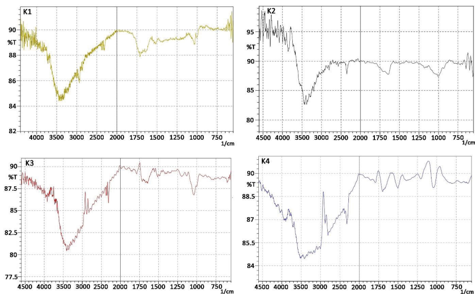
Fig. 3. Fourier-transform infrared spectrums of various humic acids isolated from Krossfjorden sediments.
