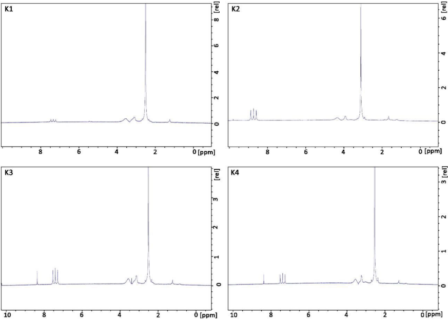
Fig. 4. 1 H Nuclear magnetic resonance spectrums of various humic acids isolated from Krossfjorden sediments.
