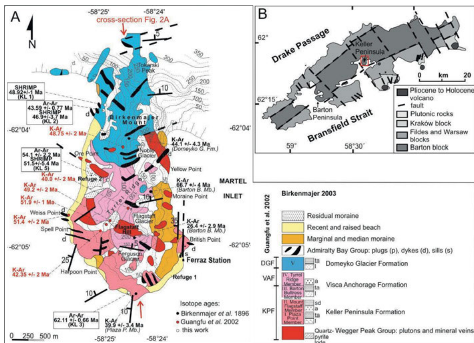
Fig. 1. (A) Geological map of the Keller Peninsula modified after Birkenmajer (2003), with locations and results of isotope dating. Topography after Mendes Júnior et al. (2012). Stratigraphic subdivision of rocks after Guangfu et al. (2002) and Birkenmajer (2003). (B) Studied area overlain by structural units of King George Island after Birkenmajer (1983).
