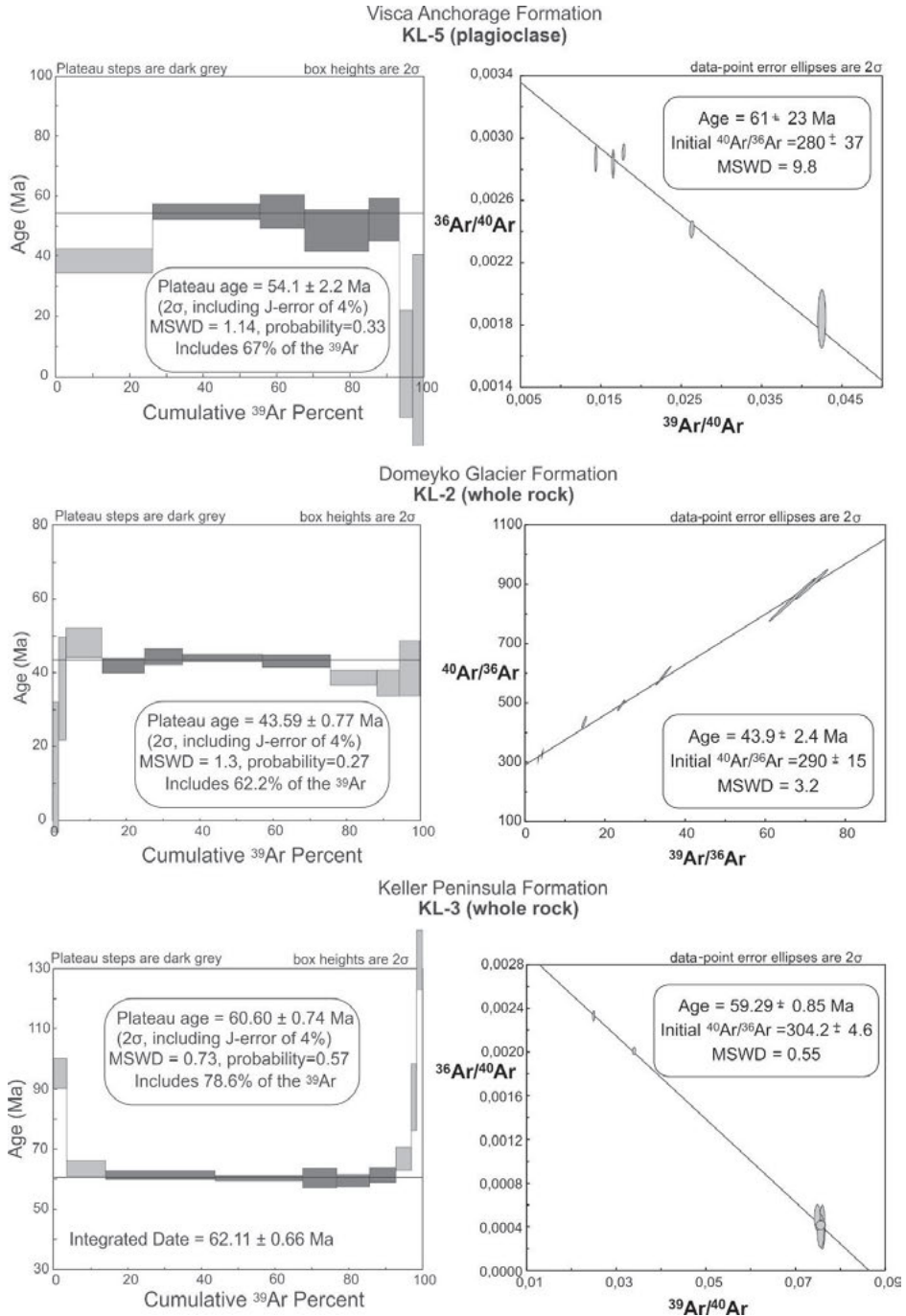
Fig. 4. Plagioclase and whole-rock sample ^{40}\text{Ar}/^{39}\text{Ar} age spectra from the volcanogenic Martel Inlet Group rocks from the Keller Peninsula presented in plateau diagrams and inverse isochron plots. The plateau age error bars of the apparent ages of step heating are drawn at 2\sigma analytical uncertainties. For details see Tables 1, 2 and 3.
