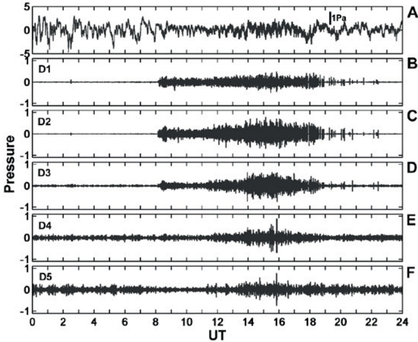
Fig. 3. Variations of atmospheric pressure (A) and wavelet decomposition levels on December 3, 2002: (B) D1 (2–4 s), (C) D2 (4–8 s), (D) D3 (8–16 s), (E) D4 (16–32 s), and (F) D5 (32–64 s).
