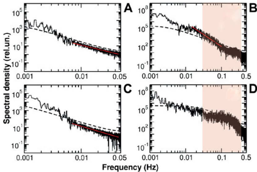
Fig. 2. MTM spectra of the atmospheric electric field (A) and atmospheric pressure (B) variations for stable conditions (01:00 to 04:00 UT of 3 December 2001) and during the fog event (14:00 to 17:00 UT of 3 December 2001) – C and D, respectively. Dashed black and solid red lines show 99% confidence levels against red noise and spectral approximations, respectively. Shaded areas show the frequency band of 0.03–0.35 Hz, in which a significant increase in pulsation intensity, more than an order of magnitude, was observed.
