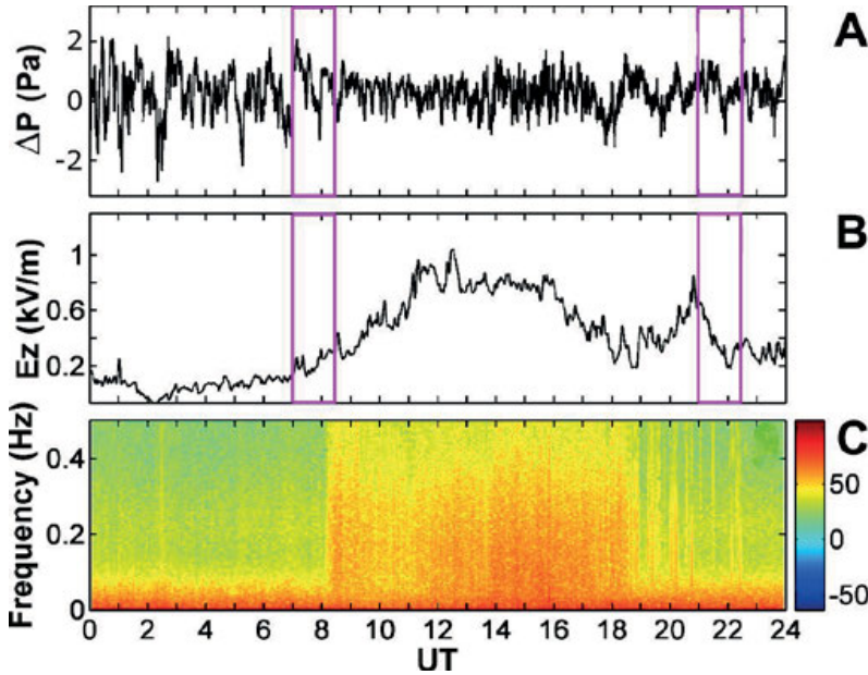
Fig. 1. Variations of atmospheric variables during the fog event of 3rd December 2001: A – atmospheric pressure (1s sampling), B – vertical electric field E_z (10s sampling), and C – spectrogram of atmospheric pressure variations. Rectangles show the intervals of fog formation and fog dissipation, respectively.
