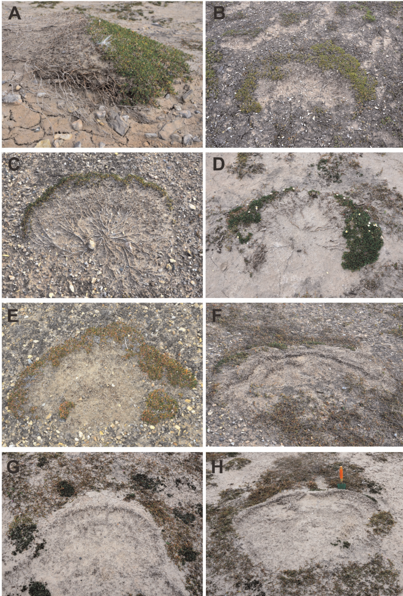
Fig. 4. Dryas aeolian landforms (DAL) development stages and variants: A – well developed mound of sediments accumulated within Dryas octopetala mat; B – wind eroded mat on the surface covered with mineral-organic crust; C – heavily eroded form on a deflationary surface; D – secondary accumulation of loose sandy deposits within eroded roots and dead shoots of Dryas octopetala ; E – stabilized mineral-organic sediments cover of DAL's eroded basin on the deflationary surface; F – same as 'E' with three successive outer micro ramparts; G – ellipsoidal DAL with two outer ramparts covered with fresh sandy deposits; H – distinct circular DAL basin refilled with fresh sandy deposits. Pictures taken in July 2012.
