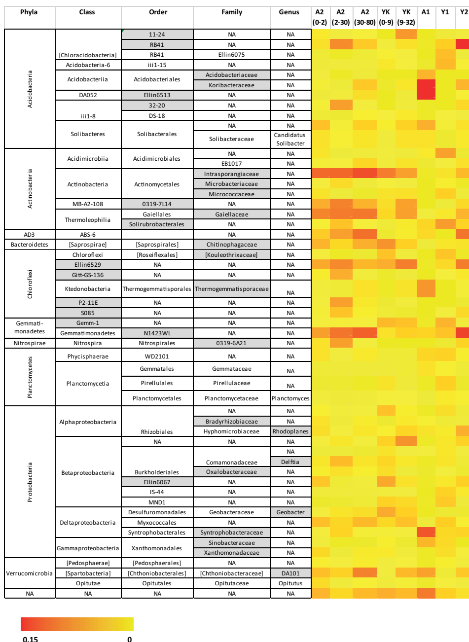
Fig. 6. Heatmap of the most abundant phylotypes for samples.
