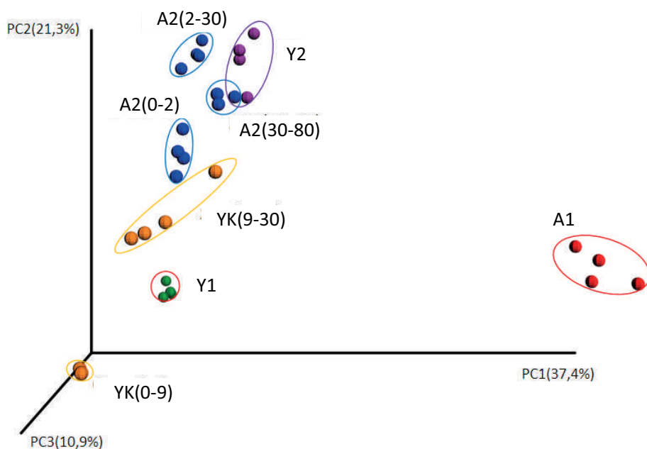
Fig. 4. Beta-diversity assessed by weighted and unweighted unifrac. PCoA for axis 1–2 and 1–3 are shown to see different dimensions.
