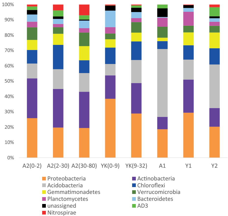
Fig. 5. Taxonomic composition of soil microbiome.
