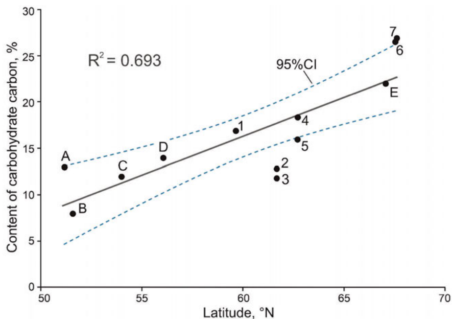
Fig. 4. Content of HA carbohydrate fragments from soil organic horizons. The steppe: A, B – Vermic Chernozems; the forest-steppe: C – Albic Luvisol; the south taiga: D, 1 – Eutric Albic Retisol (Loamic, Ochric); the middle taiga: 2 – Eutric Albic Retisol (Loamic), 3 – Eutric Albic Stagnic Histic Retisol (Loamic); the north taiga: 4 – Eutric Albic Stagnic Retisol (Loamic), 5 – Eutric Albic Stagnic Histic Retisol (Loamic); the south tundra: 6 – Stagnic Cambisol, 7 – Histic Gleysol. A, B, C, D – data after Kholodov et al. (2011), E – Hemic Follic Cryic Histosol (Vasilevich et al. 2018).
