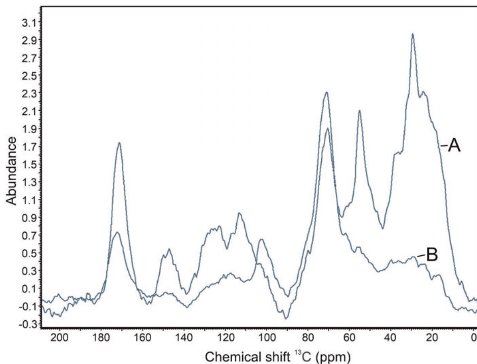
Fig. 2. CP/MAS ^{13}\text{C} NMR spectra of HAs (A) and FAs (B) isolated from the north taiga Eutric Albic Stagnic Retisol (Loamic).
