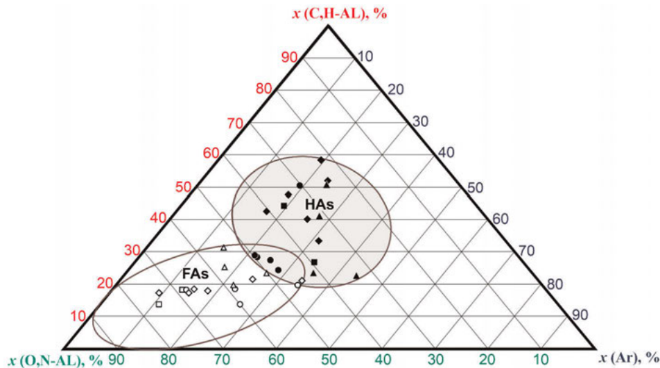
Fig. 3. Diagram of structural and functional composition of HSs from soils. The south taiga: HAs – black squares, FAs – white squares; the middle taiga: HAs – black triangles, FAs – white triangles; the north taiga: HAs – black diamonds, FAs – white diamonds; the south tundra: HAs – black circles, FAs – white circles.
