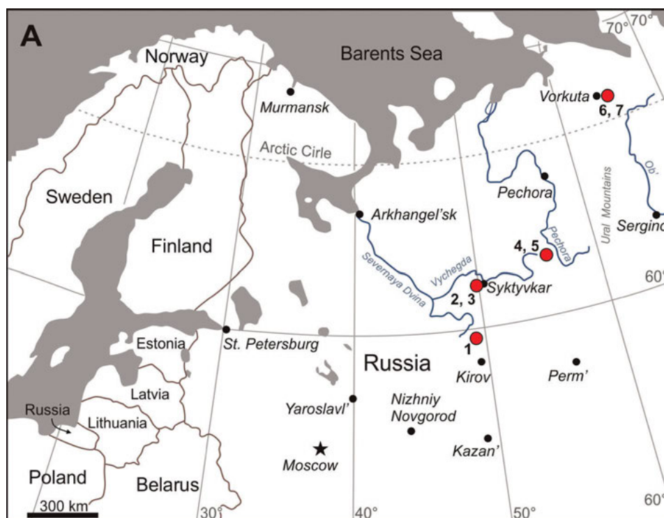
Fig. 1. Locations of sampling points. The south taiga: 1 – Eutric Albic Retisol (Loamic, Ochric); the middle taiga: 2 – Eutric Albic Retisol (Loamic), 3 – Eutric Albic Stagnic Histic Retisol (Loamic); the north taiga: 4 – Eutric Albic Stagnic Retisol (Loamic), 5 – Eutric Albic Stagnic Histic Retisol (Loamic); the south tundra: 6 – Stagnic Cambisol, 7 – Histic Gleysol.
