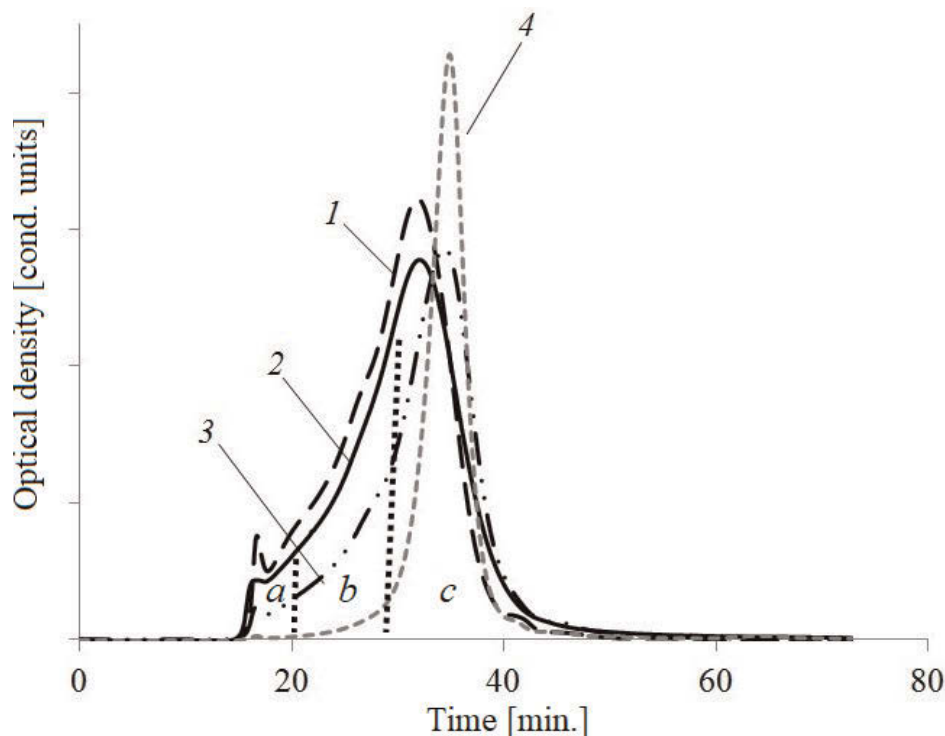
Fig. 4. Gel chromatograms of the humic acids from Histic Gleysol (1), virgin Gleyic Stagnosol (2), antropogenically altered Gleyic Stagnosol (3) and the FAs from antropogenically altered Gleyic Stagnosol (4). Where a range – high indicates molecular weight fraction, b range – medium molecular weight fraction and c range – low molecular weight fraction.
