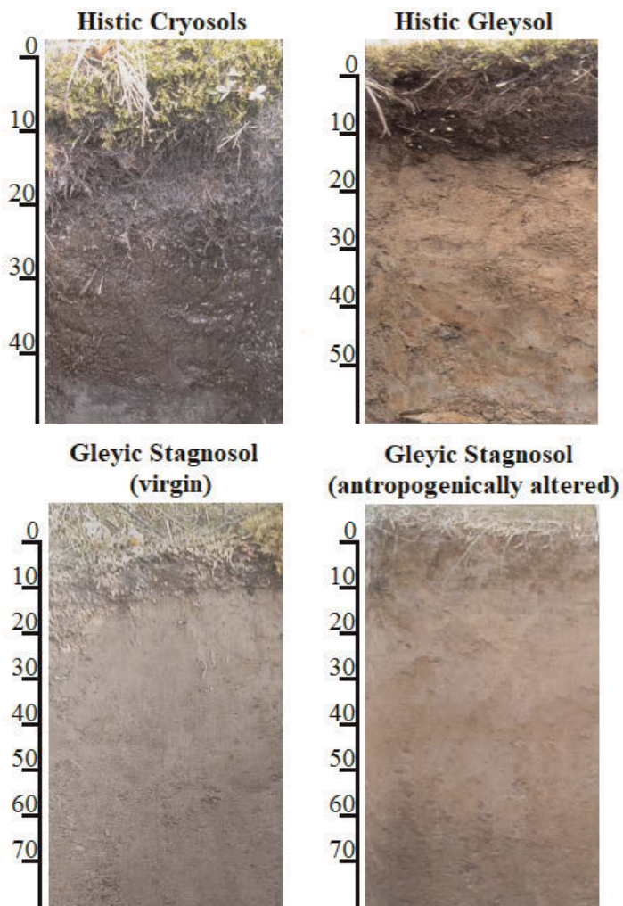
Fig. 2. Soil profiles with depths marked in cm.
