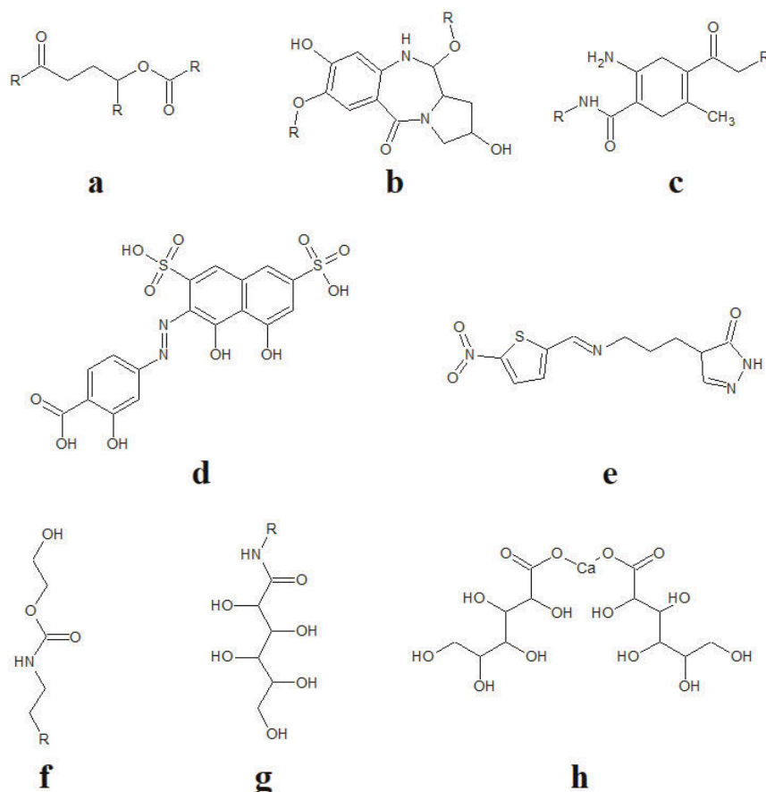
Fig. 5. The structures ( a – h ) found in humic acid samples after Tikhova et al. (2019).
