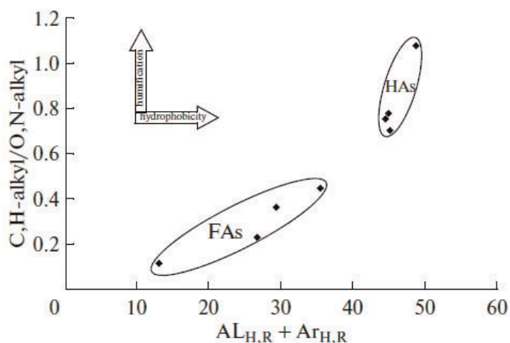
Fig. 3. Diagram of the molecular structure integrated parameters of the humic acids (HAs) and fulvic acids (FAs) from the tundra soils.
