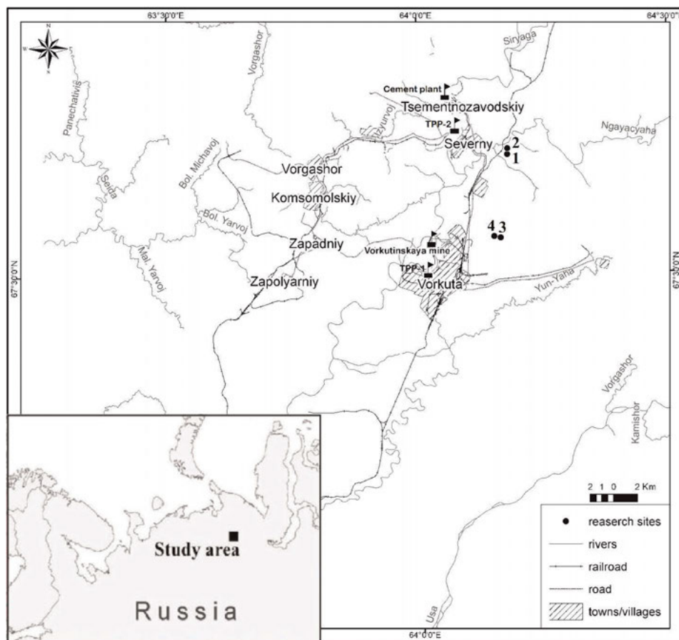
Fig. 1. Sampling locations in the Vorkuta area: 1 – Histic Cryosol, 2 – Histic Gleysol, 3 – virgin Gleyic Stagnosol and 4 – antropogenically altered Gleyic Stagnosol.
