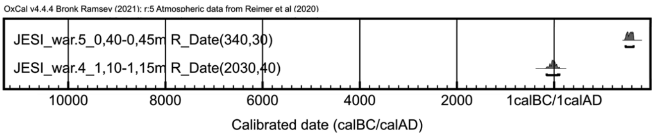
Fig. 11. Calibrated radiocarbon dates: human bone from borehole Jesi 5 (depth 0.40–0.45 m; 340 \pm 30 BP; 1474–1638 AD) and charcoal from borehole Jesi 4 (depth 1.10–1.15 m; 2030 \pm 40 BP; 153 BC–79 AD, 94.6%, and 100–107 AD, 0.9%). Calibration performed using OxCal v4.4 (Bronk Ramsey, 2009) and the IntCal20 calibration curve (Reimer et al. , 2020) at the Radiocarbon Laboratory in Poznań (drawing: F. Welc).
